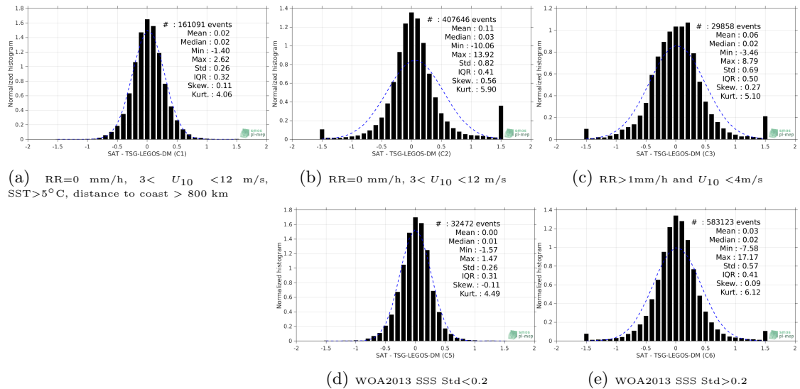
Figure 13: Normalized histogram of \Delta SSS (SMOS-L3-CATDS-CECOS-LOCEAN-V4-9DAYS-25KM - TSG-LEGOS-DM) for 5 different subdatasets corresponding to: RR=0 mm/h, 3 < U_{10} < 12 m/s, SST >5^\circ C, distance to coast > 800 km (a), RR=0 mm/h, 3 < U_{10} < 12 m/s (b), RR >1 mm/h and U_{10} < 4 m/s (c), WOA2013 SSS Std <0.2 (d), WOA2013 SSS Std >0.2 (e).
