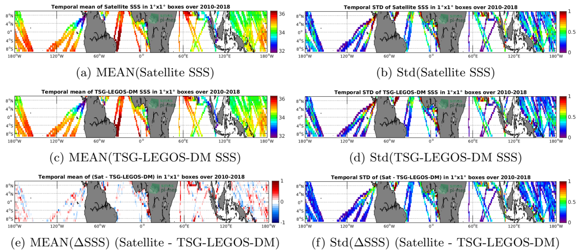
Figure 6: Temporal mean (left) and Std (right) of SSS from SMOS-L3-CATDS-CECOS-LOCEAN-V4-9DAYS-25KM (top), TSG-LEGOS-DM (middle), and of \Delta SSS (Satellite - TSG-LEGOS-DM). Only match-up pairs are used to generate these maps.
