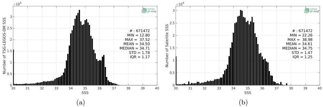
Figure 2: Histograms of SSS from TSG-LEGOS-DM (a) and SMOS-L3-CATDS-CECOS-LOCEAN-V4-9DAYS-25KM (b) considering all match-up pairs per bins of 0.1 over the Equatorial Ocean 10N-10S Pi-MEP region and for the full satellite product period.
