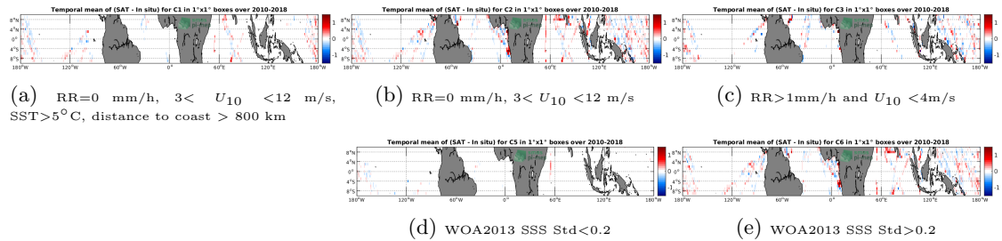
Figure 12: Temporal mean gridded over spatial boxes of size 1^\circ \times 1^\circ of \Delta SSS (SMOS-L3-CATDS-CECOS-LOCEAN-V4-9DAYS-25KM - TSG-LEGOS-DM) for 5 different subdatasets corresponding to:RR=0 mm/h, 3 < U_{10} < 12 m/s, SST >5^\circ C, distance to coast > 800 km (a), RR=0 mm/h, 3 < U_{10} < 12 m/s (b), RR >1 mm/h and U_{10} < 4 m/s (c), WOA2013 SSS Std <0.2 (d), WOA2013 SSS Std >0.2 (e).
