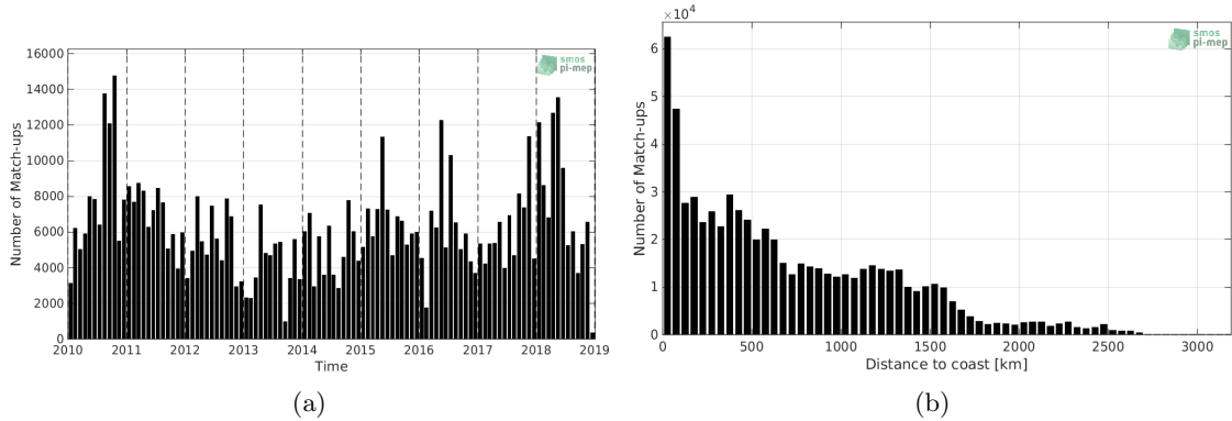
Figure 1: Number of match-ups between TSG-LEGOS-DM and SMOS-L3-CATDS-CECOS-LOCEAN-V4-9DAYS-25KM SSS as a function of time (a) and as function of the distance to coast (b) over the Equatorial Ocean 10N-10S Pi-MEP region and for the full satellite product period.
