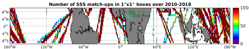
Figure 4: Number of SSS match-ups between TSG-LEGOS-DM SSS and the SMOS-L3-CATDS-CECOS-LOCEAN-V4-9DAYS-25KM SSS product for the Equatorial Ocean 10N-10S Pi-MEP region over 1°x1° boxes and for the full satellite product period.
