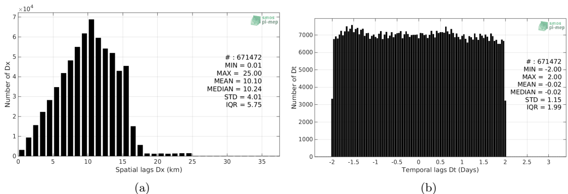
Figure 5: Histograms of the spatial (a) and temporal (b) lags between the time of the TSG-LEGOS-DM measurements and the date of the corresponding SMOS-L3-CATDS-CECOS-LOCEAN-V4-9DAYS-25KM SSS product.
