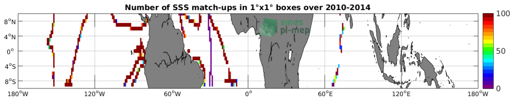
Figure 4: Number of SSS match-ups between TSG-GOSUD-Sailing-ship SSS and the SMOS-L3-CATDS-CECOS-LOCEAN-V4-9DAYS-25KM SSS product for the Equatorial Ocean 10N-10S Pi-MEP region over 1^\circ \times 1^\circ boxes and for the full satellite product period.
