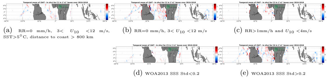
Figure 12: Temporal mean gridded over spatial boxes of size 1^\circ \times 1^\circ of \Delta SSS (SMOS SSS L3 v4 - 9 Days (CATDS-CECOS-LOCEAN) - TSG (GOSUD-Research-vessel)) for 5 different subdatasets corresponding to: RR=0 mm/h, 3 < U_{10} < 12 m/s, SST > 5^\circ\text{C} , distance to coast > 800 km (a), RR=0 mm/h, 3 < U_{10} < 12 m/s (b), RR > 1 mm/h and U_{10} < 4 m/s (c), WOA2013 SSS Std < 0.2 (d), WOA2013 SSS Std > 0.2 (e).
