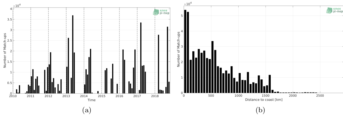
Figure 1: Number of match-ups between TSG (GOSUD-Research-vessel) and SMOS SSS L3 v4 - 9 Days (CATDS-CECOS-LOCEAN) SSS as a function of time (a) and as function of the distance to coast (b) over the Equatorial Ocean 10N-10S Pi-MEP region and for the full satellite product period.
