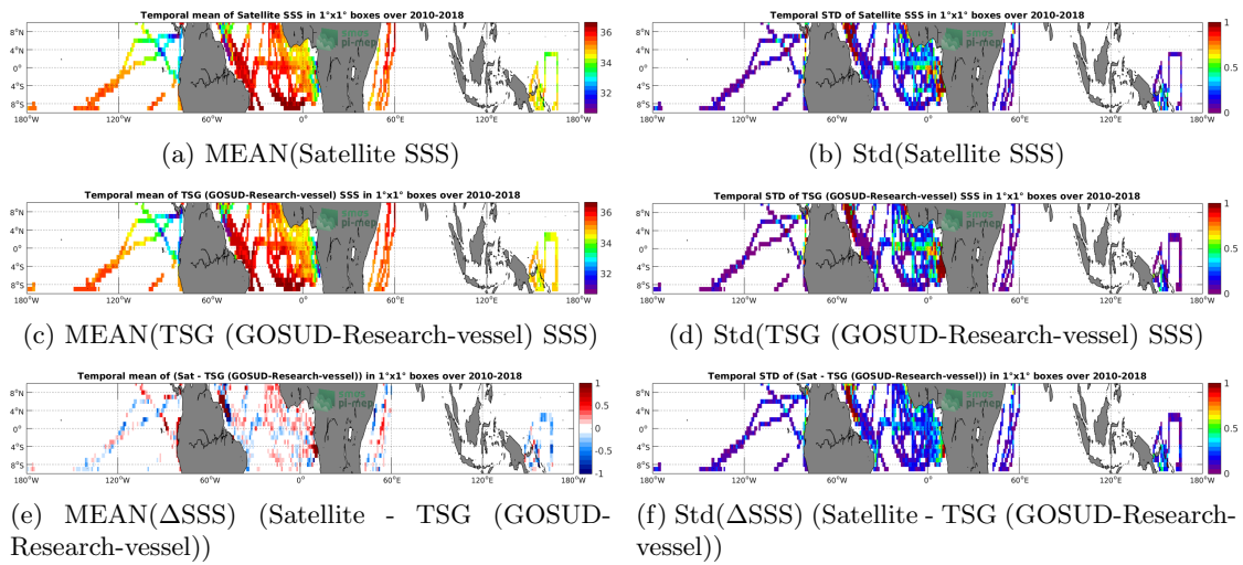
Figure 6: Temporal mean (left) and Std (right) of SSS from SMOS SSS L3 v4 - 9 Days (CATDS-CECOS-LOCEAN) (top), TSG (GOSUD-Research-vessel) (middle), and of \Delta SSS (Satellite - TSG (GOSUD-Research-vessel)). Only match-up pairs are used to generate these maps.
