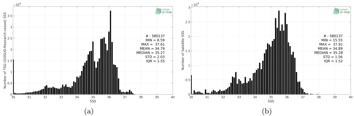
Figure 2: Histograms of SSS from TSG (GOSUD-Research-vessel) (a) and SMOS SSS L3 v4 - 9 Days (CATDS-CECOS-LOCEAN) (b) considering all match-up pairs per bins of 0.1 over the Equatorial Ocean 10N-10S Pi-MEP region and for the full satellite product period.
