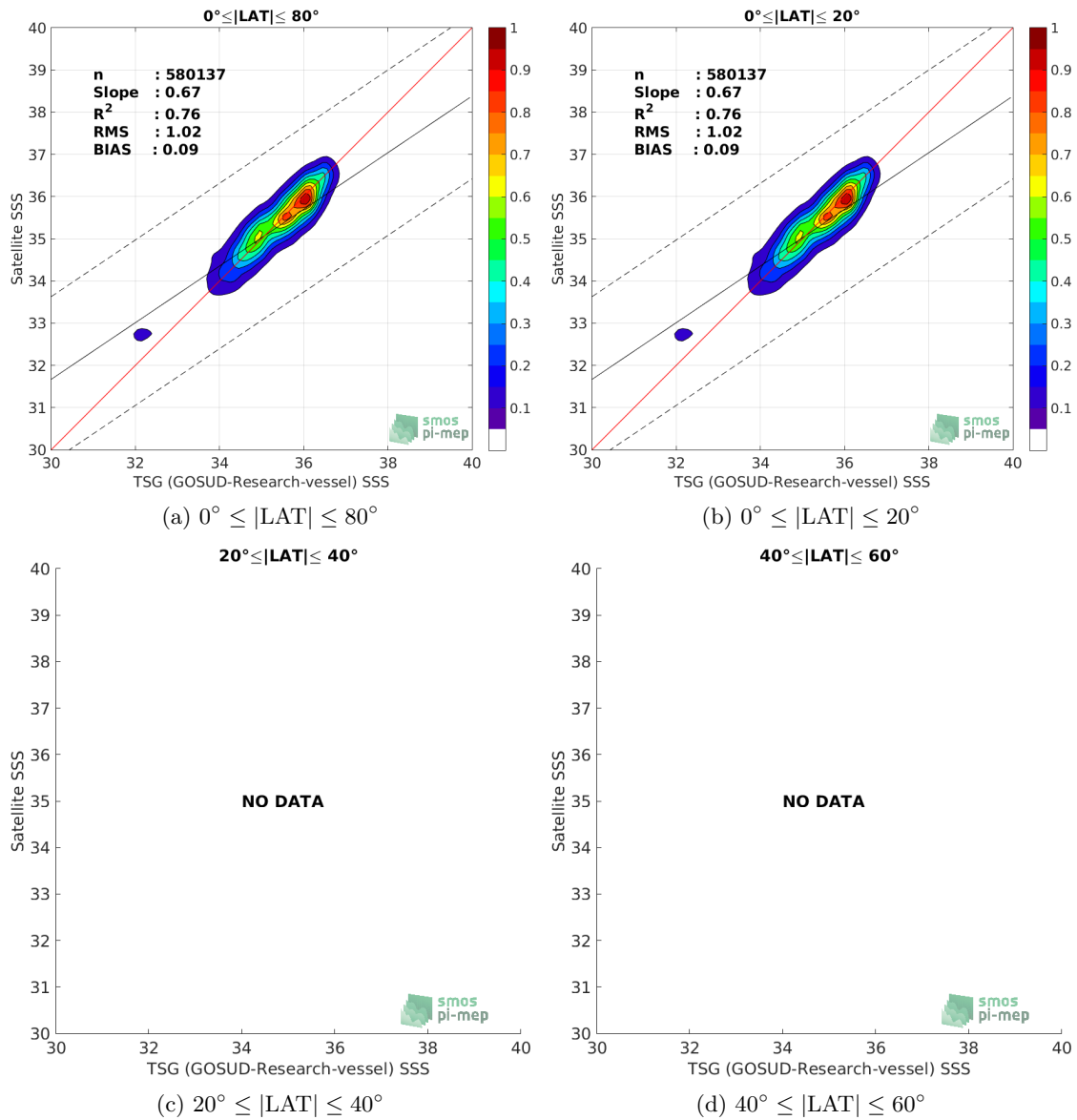
Figure 9: Contour maps of the concentration of SMOS SSS L3 v4 - 9 Days (CATDS-CECOS-LOCEAN) SSS ( y -axis) versus TSG (GOSUD-Research-vessel) SSS ( x -axis) at match-up pairs for different latitude bands. For each plot, the red line shows x=y . The black thin and dashed lines indicate a linear fit through the data cloud and the \pm 95\% confidence levels, respectively. The number match-up pairs n , the slope and R^2 coefficient of the linear fit, the root mean square (RMS) and the mean bias between satellite and in situ data are indicated for each latitude band in each plots.
