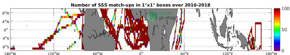
Figure 4: Number of SSS match-ups between TSG (GOSUD-Research-vessel) SSS and the SMOS SSS L3 v4 - 9 Days (CATDS-CECOS-LOCEAN) SSS product for the Equatorial Ocean 10N-10S Pi-MEP region over 1^\circ \times 1^\circ boxes and for the full satellite product period.
