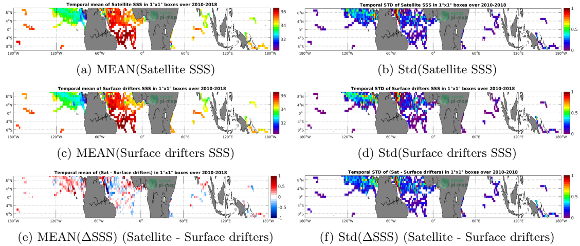
Figure 5: Temporal mean (left) and Std (right) of SSS from SMOS SSS L3 v4 - 9 Days (CATDS-CECOS-LOCEAN) (top), Surface drifters (middle), and of \Delta SSS (Satellite - Surface drifters). Only match-up pairs are used to generate these maps.
