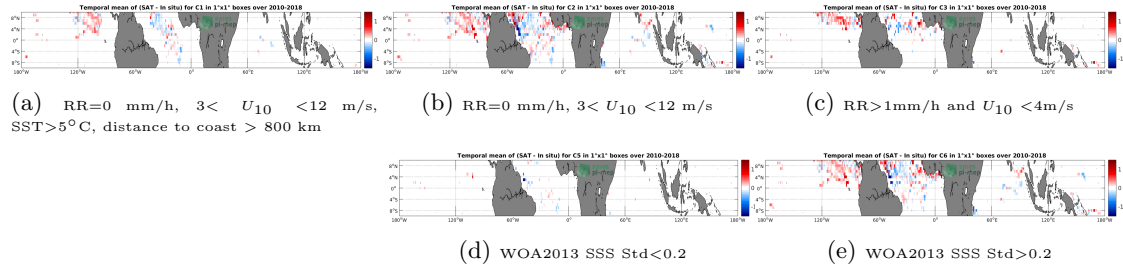
Figure 11: Temporal mean gridded over spatial boxes of size 1^{\circ}\times 1^{\circ} of \Delta\text{SSS} (SMOS SSS L3 v4 - 9 Days (CATDS-CECOS-LOCEAN) - Surface drifters) for 5 different subdatasets corresponding to:RR=0 mm/h, 3 < U_{10} < 12 m/s, SST >5^{\circ}\text{C} , distance to coast > 800 km (a), RR=0 mm/h, 3 < U_{10} < 12 m/s (b), RR >1 mm/h and U_{10} < 4 m/s (c), WOA2013 SSS Std <0.2 (d), WOA2013 SSS Std >0.2 (e).
