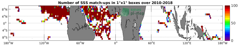
Figure 3: Number of SSS match-ups between Surface drifters SSS and the SMOS SSS L3 v4 - 9 Days (CATDS-CECOS-LOCEAN) SSS product for the Equatorial Ocean 10N-10S Pi-MEP region over 1^\circ \times 1^\circ boxes and for the full satellite product period.
