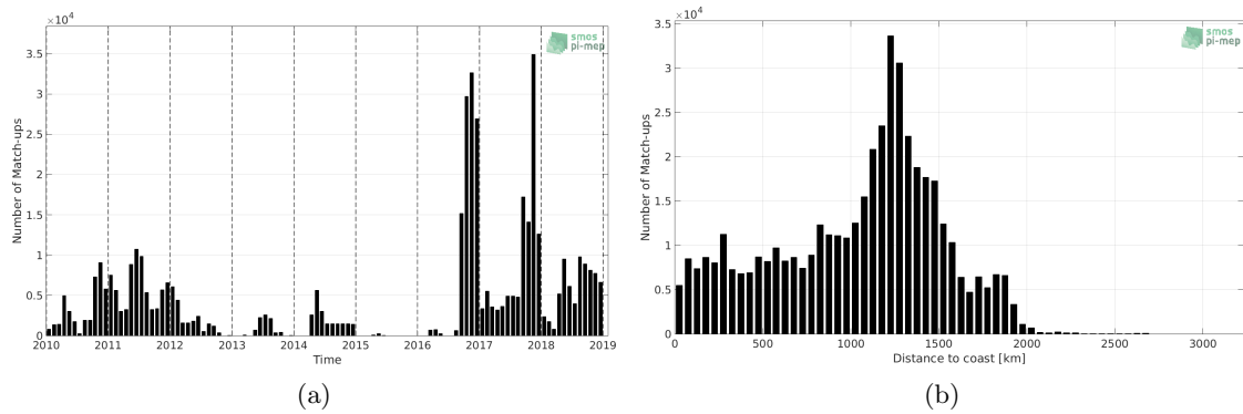
Figure 1: Number of match-ups between Surface drifters and SMOS SSS L3 v4 - 9 Days (CATDS-CECOS-LOCEAN) SSS as a function of time (a) and as function of the distance to coast (b) over the Equatorial Ocean 10N-10S Pi-MEP region and for the full satellite product period.
