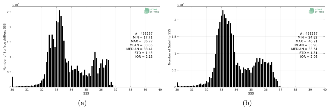
Figure 2: Histograms of SSS from Surface drifters (a) and SMOS SSS L3 v4 - 9 Days (CATDS-CECOS-LOCEAN) (b) considering all match-up pairs per bins of 0.1 over the Equatorial Ocean 10N-10S Pi-MEP region and for the full satellite product period.
