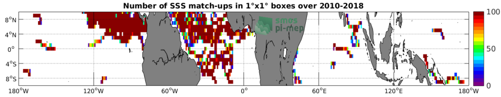
Figure 3: Number of SSS match-ups between Surface drifters SSS and the SMOS-L3-CATDS-CECOS-LOCEAN-V4-9DAYS-25KM SSS product for the Equatorial Ocean 10N-10S Pi-MEP region over 1^\circ \times 1^\circ boxes and for the full satellite product period.
