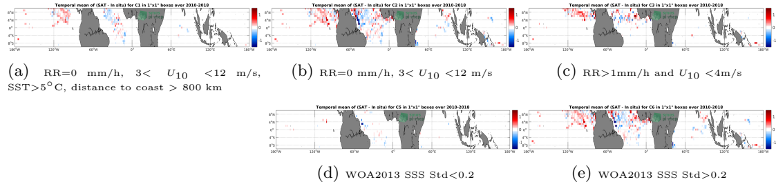
Figure 11: Temporal mean gridded over spatial boxes of size 1^{\circ}\times 1^{\circ} of \Delta\text{SSS} (SMOS-L3-CATDS-CECOS-LOCEAN-V4-9DAYS-25KM - Surface drifters) for 5 different subdatasets corresponding to:RR=0 mm/h, 3 < U_{10} < 12 m/s, SST >5^{\circ}\text{C} , distance to coast > 800 km (a), RR=0 mm/h, 3 < U_{10} < 12 m/s (b), RR >1 mm/h and U_{10} < 4 m/s (c), WOA2013 SSS Std <0.2 (d), WOA2013 SSS Std >0.2 (e).
