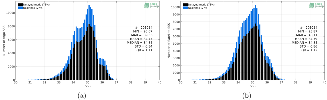
Figure 2: Histograms of SSS from Argo (a) and SMOS-L3-CATDS-CECOS-LOCEAN-V4-9DAYS-25KM (b) considering all match-up pairs per bins of 0.1 over the Equatorial Ocean 10N-10S Pi-MEP region and for the full satellite product period.
