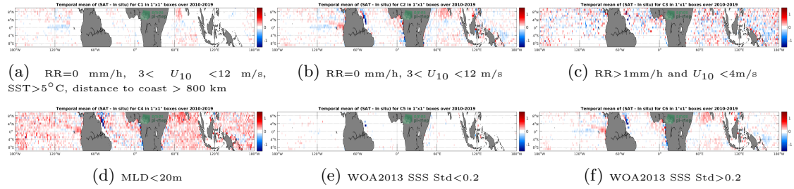
Figure 12: Temporal mean gridded over spatial boxes of size 1^\circ \times 1^\circ of \Delta SSS (SMOS-L3-CATDS-CECOS-LOCEAN-V4-9DAYS-25KM - Argo) for 6 different subdatasets corresponding to: RR=0 mm/h, 3 < U_{10} < 12 m/s, SST > 5^\circ C , distance to coast > 800 km (a), RR=0 mm/h, 3 < U_{10} < 12 m/s (b), RR > 1 mm/h and U_{10} < 4 m/s (c), MLD < 20 m (d), WOA2013 SSS Std < 0.2 (e), WOA2013 SSS Std > 0.2 (f).
