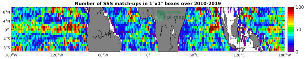
Figure 4: Number of SSS match-ups between Argo SSS and the SMOS-L3-CATDS-CECOS-LOCEAN-V4-9DAYS-25KM SSS product for the Equatorial Ocean 10N-10S Pi-MEP region over 1°x1° boxes and for the full satellite product period.
