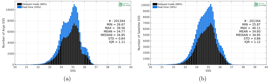
Figure 2: Histograms of SSS from Argo (a) and SMOS-L3-CATDS-CECOS-LOCEAN-V4-9DAYS-25KM (b) considering all match-up pairs per bins of 0.1 over the Equatorial Ocean 10N-10S Pi-MEP region and for the full satellite product period.
