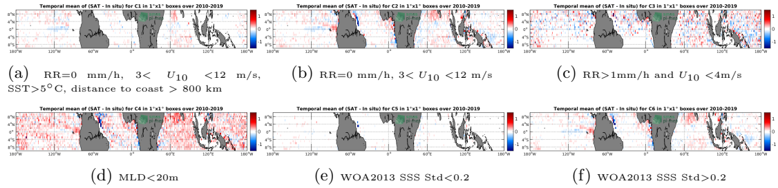
Figure 12: Temporal mean gridded over spatial boxes of size 1^\circ \times 1^\circ of \Delta SSS (SMOS-L3-CATDS-CECOS-LOCEAN-V4-9DAYS-25KM - Argo) for 6 different subdatasets corresponding to: RR=0 mm/h, 3 < U_{10} < 12 m/s, SST >5^\circ\text{C} , distance to coast > 800 km (a), RR=0 mm/h, 3 < U_{10} < 12 m/s (b), RR >1 mm/h and U_{10} < 4 m/s (c),MLD <20 m (d),WOA2013 SSS Std <0.2 (e),WOA2013 SSS Std >0.2 (f).
