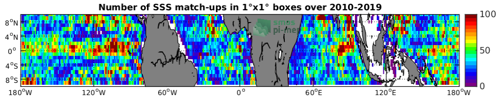
Figure 4: Number of SSS match-ups between Argo SSS and the SMOS-L3-CATDS-CECOS-LOCEAN-V4-9DAYS-25KM SSS product for the Equatorial Ocean 10N-10S Pi-MEP region over 1°x1° boxes and for the full satellite product period.
