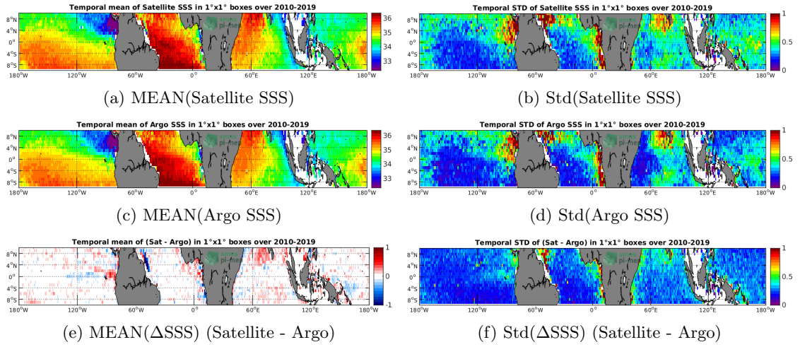
Figure 6: Temporal mean (left) and Std (right) of SSS from SMOS-L3-CATDS-CECOS-LOCEAN-V4-9DAYS-25KM (top), Argo (middle), and of \Delta SSS (Satellite - Argo). Only match-up pairs are used to generate these maps.
