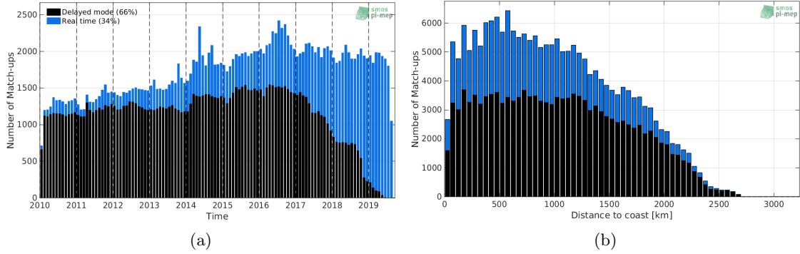
Figure 1: Number of match-ups between Argo and SMOS-L3-CATDS-CECOS-LOCEAN-V4-9DAYS-25KM SSS as a function of time (a) and as function of the distance to coast (b) over the Equatorial Ocean 10N-10S Pi-MEP region and for the full satellite product period.
