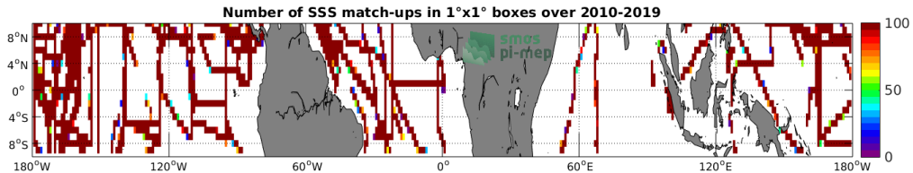
Figure 4: Number of SSS match-ups between TSG (SAMOS) SSS and the SMOS SSS L3 v4 - 18 Days (CATDS-CECOS-LOCEAN) SSS product for the Equatorial Ocean 10N-10S Pi-MEP region over 1°x1° boxes and for the full satellite product period.
