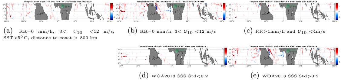
Figure 12: Temporal mean gridded over spatial boxes of size 1^{\circ}\times 1^{\circ} of \Delta\text{SSS} (SMOS SSS L3 v4 - 18 Days (CATDS-CECOS-LOCEAN) - TSG (SAMOS)) for 5 different subdatasets corresponding to: \text{RR}=0 \text{ mm/h} , 3 < U_{10} < 12 \text{ m/s} , \text{SST} > 5^{\circ}\text{C} , distance to coast > 800 \text{ km} (a), \text{RR}=0 \text{ mm/h} , 3 < U_{10} < 12 \text{ m/s} (b), \text{RR} > 1 \text{ mm/h} and U_{10} < 4 \text{ m/s} (c), WOA2013 SSS Std < 0.2 (d), WOA2013 SSS Std > 0.2 (e).
