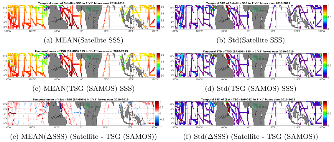
Figure 6: Temporal mean (left) and Std (right) of SSS from SMOS SSS L3 v4 - 18 Days (CATDS-CECOS-LOCEAN) (top), TSG (SAMOS) (middle), and of \Delta SSS (Satellite - TSG (SAMOS)). Only match-up pairs are used to generate these maps.
