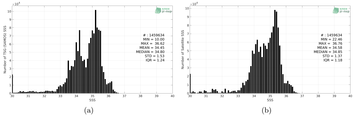
Figure 2: Histograms of SSS from TSG (SAMOS) (a) and SMOS SSS L3 v4 - 18 Days (CATDS-CECOS-LOCEAN) (b) considering all match-up pairs per bins of 0.1 over the Equatorial Ocean 10N-10S Pi-MEP region and for the full satellite product period.
