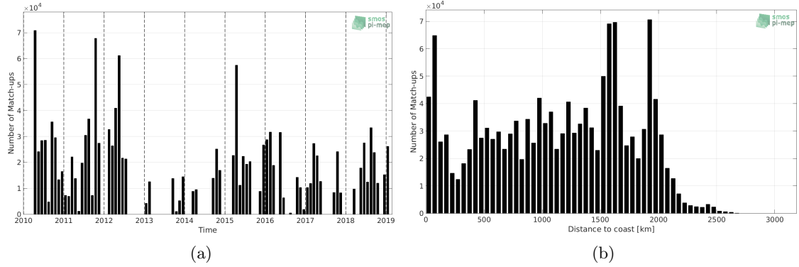
Figure 1: Number of match-ups between TSG (SAMOS) and SMOS SSS L3 v4 - 18 Days (CATDS-CECOS-LOCEAN) SSS as a function of time (a) and as function of the distance to coast (b) over the Equatorial Ocean 10N-10S Pi-MEP region and for the full satellite product period.
