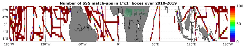
Figure 4: Number of SSS match-ups between TSG-SAMOS SSS and the SMOS-L3-CATDS-CECOS-LOCEAN-V4-18DAYS-25KM SSS product for the Equatorial Ocean 10N-10S Pi-MEP region over 1°x1° boxes and for the full satellite product period.
