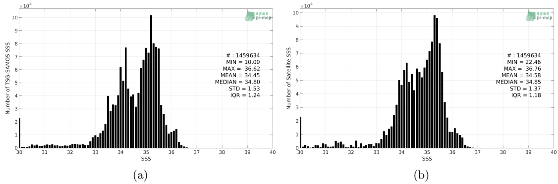
Figure 2: Histograms of SSS from TSG-SAMOS (a) and SMOS-L3-CATDS-CECOS-LOCEAN-V4-18DAYS-25KM (b) considering all match-up pairs per bins of 0.1 over the Equatorial Ocean 10N-10S Pi-MEP region and for the full satellite product period.
