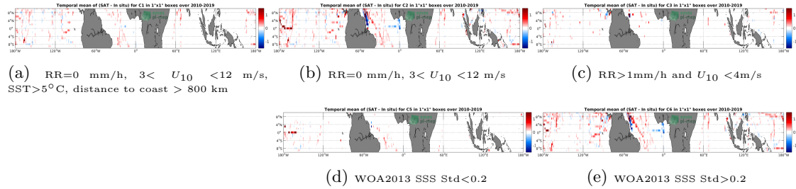
Figure 12: Temporal mean gridded over spatial boxes of size 1^{\circ}\times 1^{\circ} of \Delta\text{SSS} (SMOS-L3-CATDS-CECOS-LOCEAN-V4-18DAYS-25KM - TSG-SAMOS) for 5 different subdatasets corresponding to: RR=0 mm/h, 3 < U_{10} < 12 m/s, SST > 5^{\circ}\text{C} , distance to coast > 800 km (a), RR=0 mm/h, 3 < U_{10} < 12 m/s (b), RR > 1 mm/h and U_{10} < 4 m/s (c), WOA2013 SSS Std < 0.2 (d), WOA2013 SSS Std > 0.2 (e).
