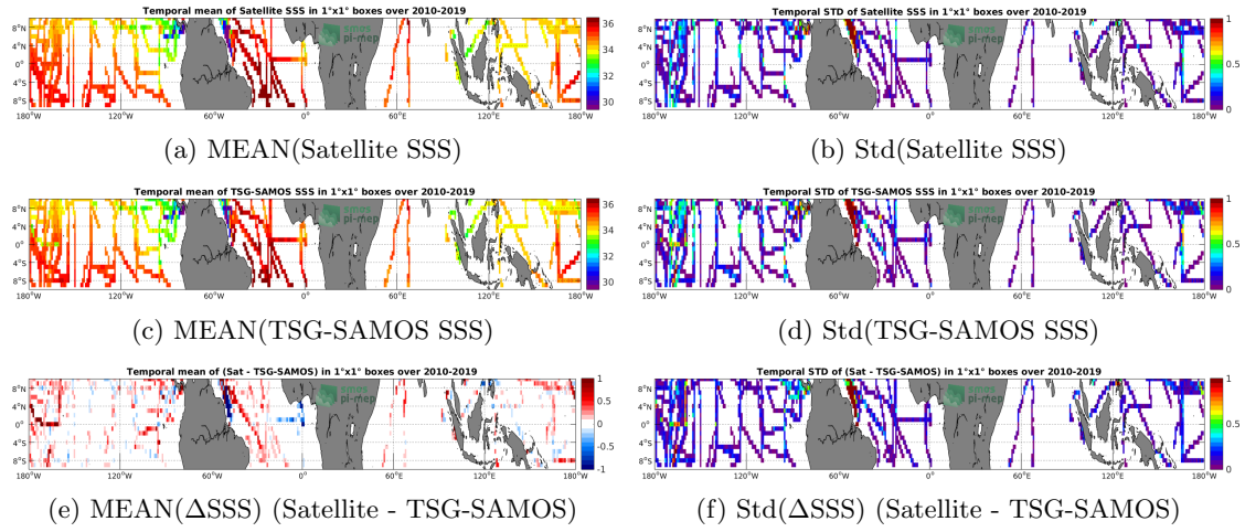
Figure 6: Temporal mean (left) and Std (right) of SSS from SMOS-L3-CATDS-CECOS-LOCEAN-V4-18DAYS-25KM (top), TSG-SAMOS (middle), and of \Delta SSS (Satellite - TSG-SAMOS). Only match-up pairs are used to generate these maps.
