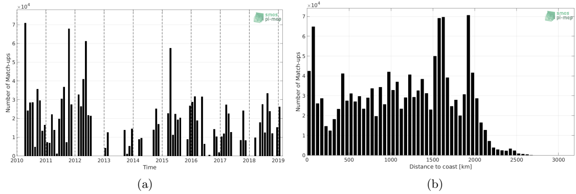
Figure 1: Number of match-ups between TSG-SAMOS and SMOS-L3-CATDS-CECOS-LOCEAN-V4-18DAYS-25KM SSS as a function of time (a) and as function of the distance to coast (b) over the Equatorial Ocean 10N-10S Pi-MEP region and for the full satellite product period.
