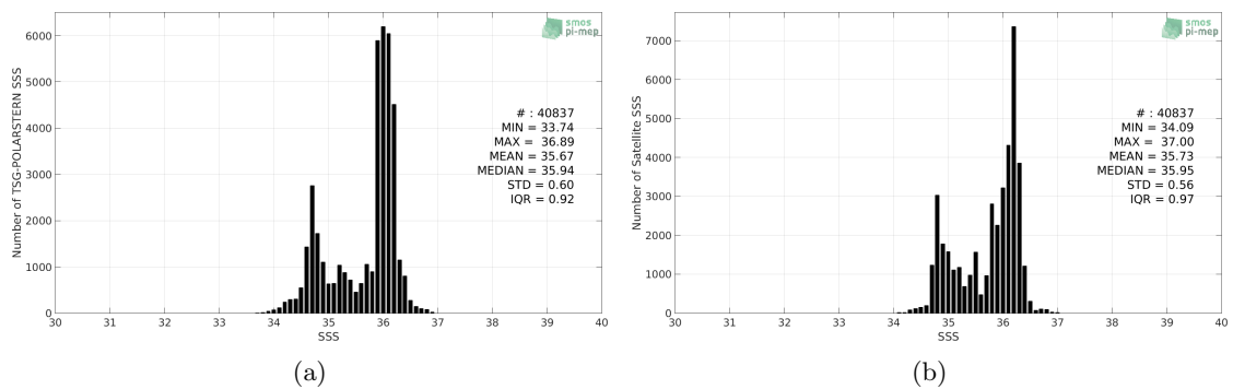
Figure 2: Histograms of SSS from TSG-POLARSTERN (a) and SMOS-L3-CATDS-CECOS-LOCEAN-V4-18DAYS-25KM (b) considering all match-up pairs per bins of 0.1 over the Equatorial Ocean 10N-10S Pi-MEP region and for the full satellite product period.
