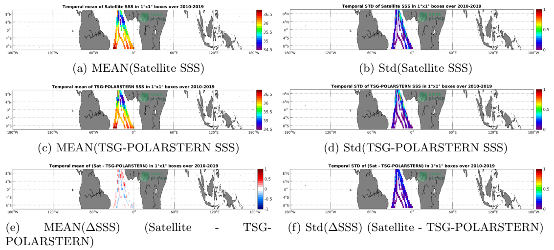
Figure 6: Temporal mean (left) and Std (right) of SSS from SMOS-L3-CATDS-CECOS-LOCEAN-V4-18DAYS-25KM (top), TSG-POLARSTERN (middle), and of \Delta SSS (Satellite - TSG-POLARSTERN). Only match-up pairs are used to generate these maps.
