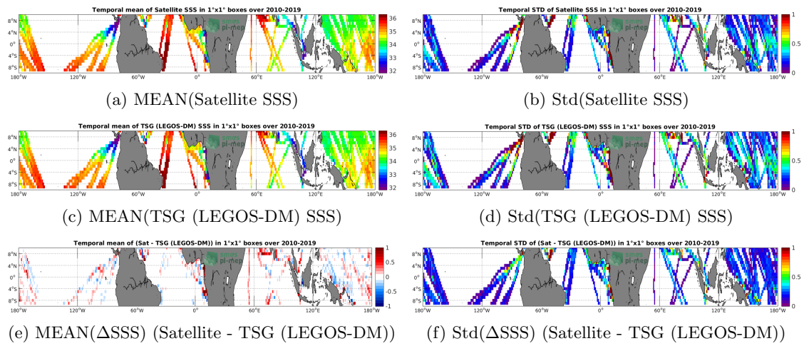
Figure 6: Temporal mean (left) and Std (right) of SSS from SMOS SSS L3 v4 - 18 Days (CATDS-CECOS-LOCEAN) (top), TSG (LEGOS-DM) (middle), and of \Delta SSS (Satellite - TSG (LEGOS-DM)). Only match-up pairs are used to generate these maps.
