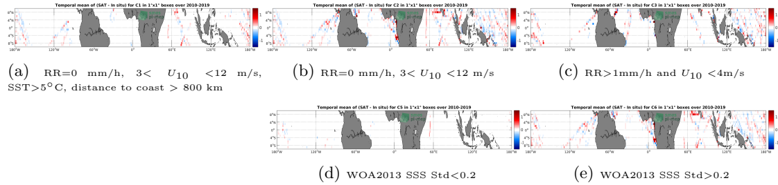
Figure 12: Temporal mean gridded over spatial boxes of size 1^{\circ}\times 1^{\circ} of \Delta\text{SSS} (SMOS SSS L3 v4 - 18 Days (CATDS-CECOS-LOCEAN) - TSG (LEGOS-DM)) for 5 different subdatasets corresponding to:RR=0 mm/h, 3 < U_{10} < 12 m/s, SST >5^{\circ}\text{C} , distance to coast > 800 km (a), RR=0 mm/h, 3 < U_{10} < 12 m/s (b), RR >1 mm/h and U_{10} < 4 m/s (c), WOA2013 SSS Std <0.2 (d), WOA2013 SSS Std >0.2 (e).
