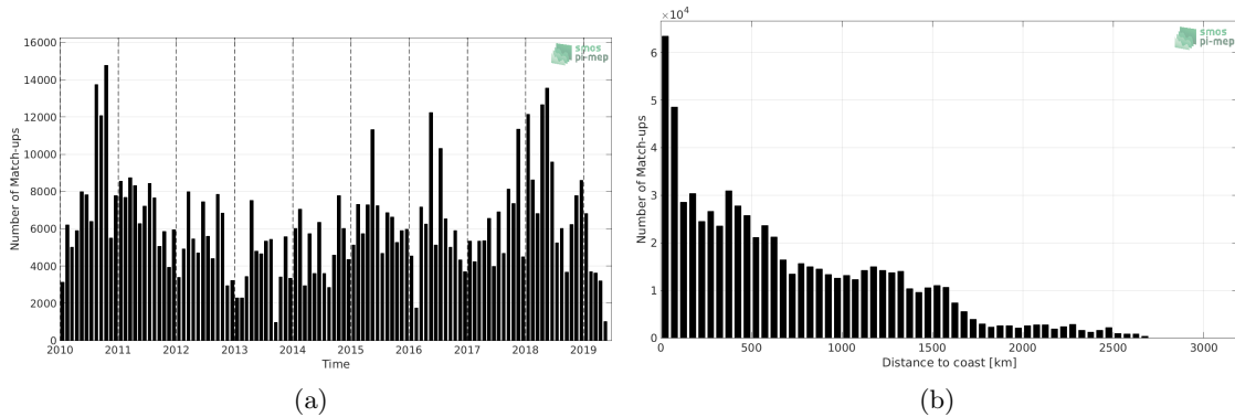
Figure 1: Number of match-ups between TSG (LEGOS-DM) and SMOS SSS L3 v4 - 18 Days (CATDS-CECOS-LOCEAN) SSS as a function of time (a) and as function of the distance to coast (b) over the Equatorial Ocean 10N-10S Pi-MEP region and for the full satellite product period.
