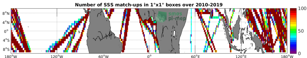
Figure 4: Number of SSS match-ups between TSG (LEGOS-DM) SSS and the SMOS SSS L3 v4 - 18 Days (CATDS-CECOS-LOCEAN) SSS product for the Equatorial Ocean 10N-10S Pi-MEP region over 1^\circ \times 1^\circ boxes and for the full satellite product period.
