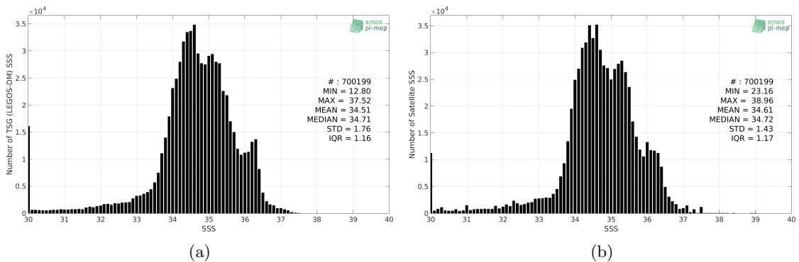
Figure 2: Histograms of SSS from TSG (LEGOS-DM) (a) and SMOS SSS L3 v4 - 18 Days (CATDS-CECOS-LOCEAN) (b) considering all match-up pairs per bins of 0.1 over the Equatorial Ocean 10N-10S Pi-MEP region and for the full satellite product period.
