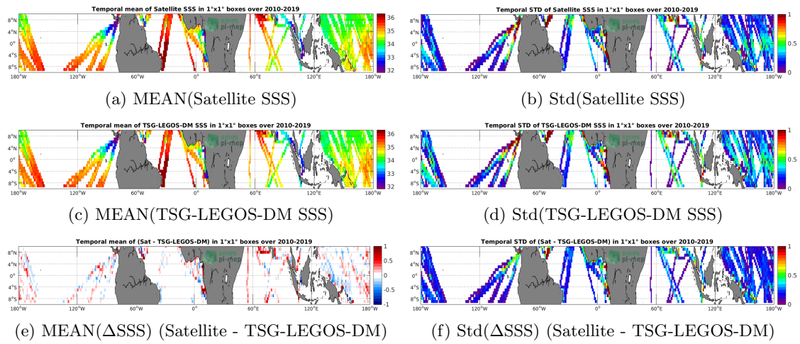
Figure 6: Temporal mean (left) and Std (right) of SSS from SMOS-L3-CATDS-CECOS-LOCEAN-V4-18DAYS-25KM (top), TSG-LEGOS-DM (middle), and of \Delta SSS (Satellite - TSG-LEGOS-DM). Only match-up pairs are used to generate these maps.
