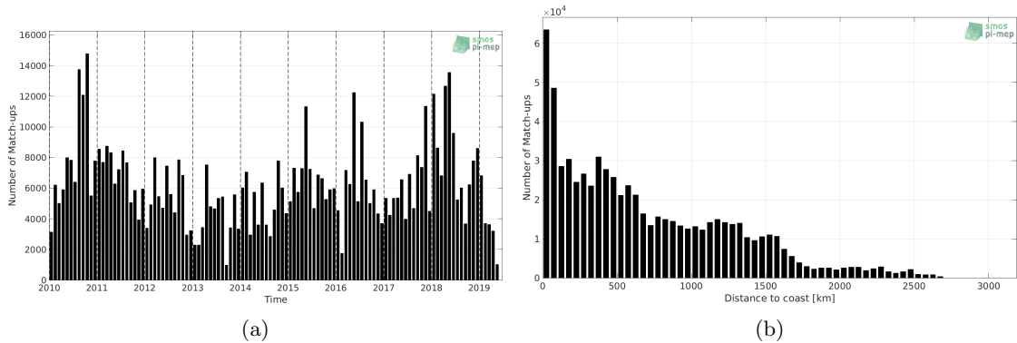
Figure 1: Number of match-ups between TSG-LEGOS-DM and SMOS-L3-CATDS-CECOS-LOCEAN-V4-18DAYS-25KM SSS as a function of time (a) and as function of the distance to coast (b) over the Equatorial Ocean 10N-10S Pi-MEP region and for the full satellite product period.
