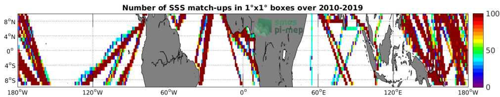
Figure 4: Number of SSS match-ups between TSG-LEGOS-DM SSS and the SMOS-L3-CATDS-CECOS-LOCEAN-V4-18DAYS-25KM SSS product for the Equatorial Ocean 10N-10S Pi-MEP region over 1^\circ \times 1^\circ boxes and for the full satellite product period.
