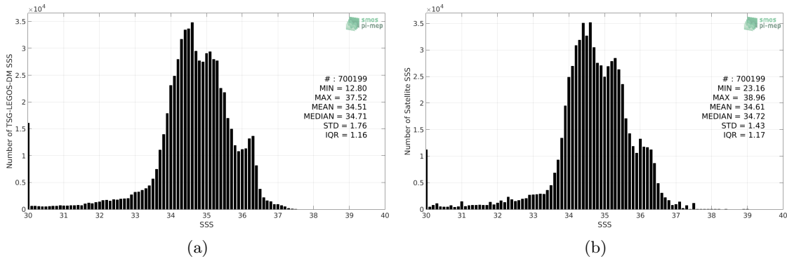
Figure 2: Histograms of SSS from TSG-LEGOS-DM (a) and SMOS-L3-CATDS-CECOS-LOCEAN-V4-18DAYS-25KM (b) considering all match-up pairs per bins of 0.1 over the Equatorial Ocean 10N-10S Pi-MEP region and for the full satellite product period.
