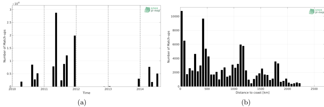
Figure 1: Number of match-ups between TSG (GOSUD-Sailing-ship) and SMOS SSS L3 v4 - 18 Days (CATDS-CECOS-LOCEAN) SSS as a function of time (a) and as function of the distance to coast (b) over the Equatorial Ocean 10N-10S Pi-MEP region and for the full satellite product period.
