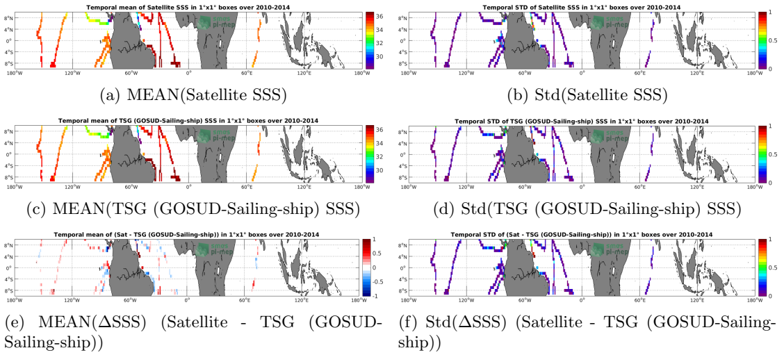
Figure 6: Temporal mean (left) and Std (right) of SSS from SMOS SSS L3 v4 - 18 Days (CATDS-CECOS-LOCEAN) (top), TSG (GOSUD-Sailing-ship) (middle), and of \Delta SSS (Satellite - TSG (GOSUD-Sailing-ship)). Only match-up pairs are used to generate these maps.
