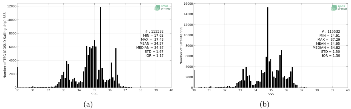
Figure 2: Histograms of SSS from TSG (GOSUD-Sailing-ship) (a) and SMOS SSS L3 v4 - 18 Days (CATDS-CECOS-LOCEAN) (b) considering all match-up pairs per bins of 0.1 over the Equatorial Ocean 10N-10S Pi-MEP region and for the full satellite product period.
