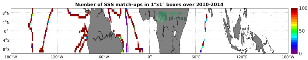
Figure 4: Number of SSS match-ups between TSG (GOSUD-Sailing-ship) SSS and the SMOS SSS L3 v4 - 18 Days (CATDS-CECOS-LOCEAN) SSS product for the Equatorial Ocean 10N-10S Pi-MEP region over 1^\circ \times 1^\circ boxes and for the full satellite product period.
