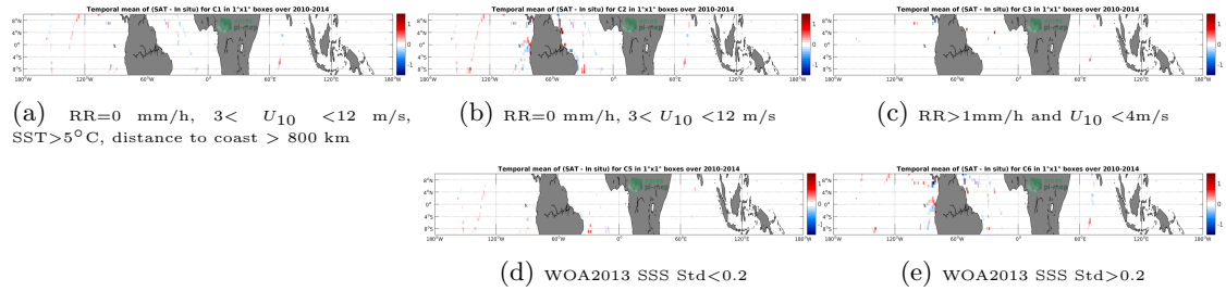
Figure 12: Temporal mean gridded over spatial boxes of size 1^{\circ}\times 1^{\circ} of \Delta SSS (SMOS-L3-CATDS-CECOS-LOCEAN-V4-18DAYS-25KM - TSG-GOSUD-Sailing-ship) for 5 different subdatasets corresponding to:RR=0 mm/h, 3 < U_{10} < 12 m/s, SST >5^{\circ}\text{C} , distance to coast > 800 km (a), RR=0 mm/h, 3 < U_{10} < 12 m/s (b), RR >1 mm/h and U_{10} < 4 m/s (c), WOA2013 SSS Std <0.2 (d), WOA2013 SSS Std >0.2 (e).
