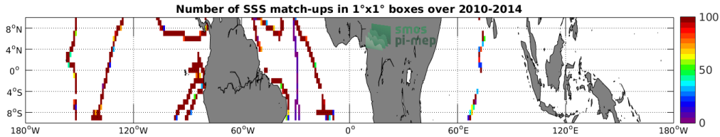
Figure 4: Number of SSS match-ups between TSG-GOSUD-Sailing-ship SSS and the SMOS-L3-CATDS-CECOS-LOCEAN-V4-18DAYS-25KM SSS product for the Equatorial Ocean 10N-10S Pi-MEP region over 1^\circ \times 1^\circ boxes and for the full satellite product period.
