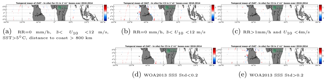
Figure 12: Temporal mean gridded over spatial boxes of size 1°x1° of \Delta SSS (SMOS-L3-CATDS-CECOS-LOCEAN-V4-18DAYS-25KM - TSG-GOSUD-Sailing-ship) for 5 different subdatasets corresponding to:RR=0 mm/h, 3 < U_{10} < 12 m/s, SST>5°C, distance to coast > 800 km (a), RR=0 mm/h, 3 < U_{10} < 12 m/s (b), RR>1mm/h and U_{10} < 4 m/s (c), WOA2013 SSS Std<0.2 (d), WOA2013 SSS Std>0.2 (e).
