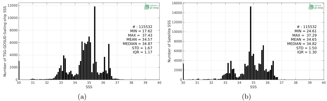
Figure 2: Histograms of SSS from TSG-GOSUD-Sailing-ship (a) and SMOS-L3-CATDS-CECOS-LOCEAN-V4-18DAYS-25KM (b) considering all match-up pairs per bins of 0.1 over the Equatorial Ocean 10N-10S Pi-MEP region and for the full satellite product period.
