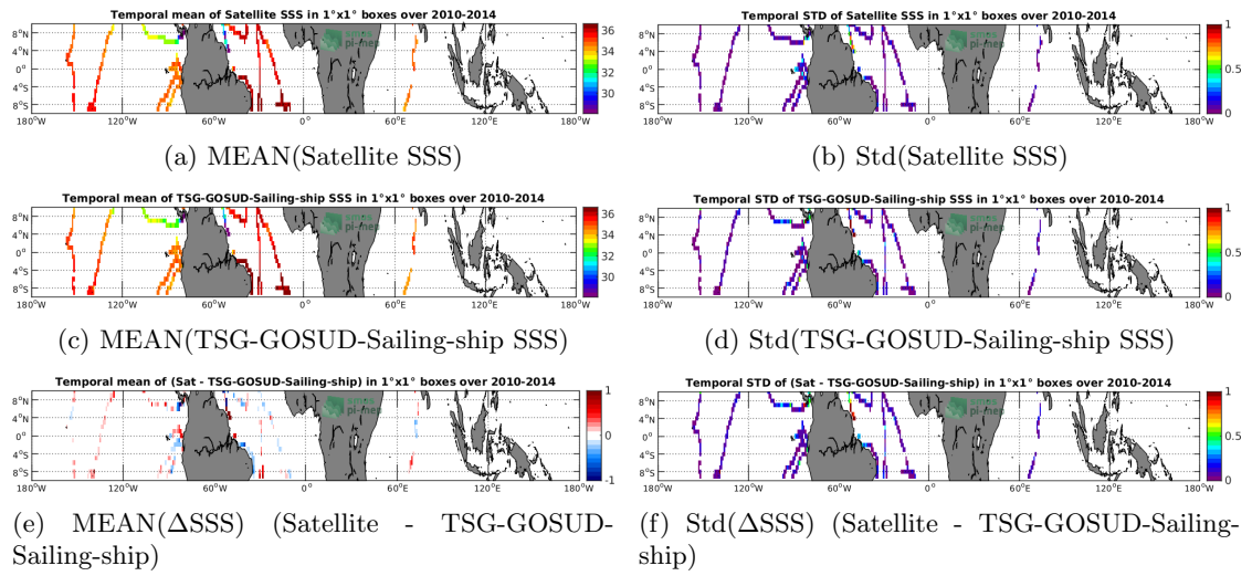
Figure 6: Temporal mean (left) and Std (right) of SSS from SMOS-L3-CATDS-CECOS-LOCEAN-V4-18DAYS-25KM (top), TSG-GOSUD-Sailing-ship (middle), and of \Delta SSS (Satellite - TSG-GOSUD-Sailing-ship). Only match-up pairs are used to generate these maps.
