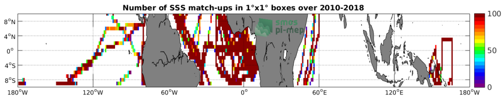
Figure 4: Number of SSS match-ups between TSG (GOSUD-Research-vessel) SSS and the SMOS SSS L3 v4 - 18 Days (CATDS-CECOS-LOCEAN) SSS product for the Equatorial Ocean 10N-10S Pi-MEP region over 1^\circ \times 1^\circ boxes and for the full satellite product period.
