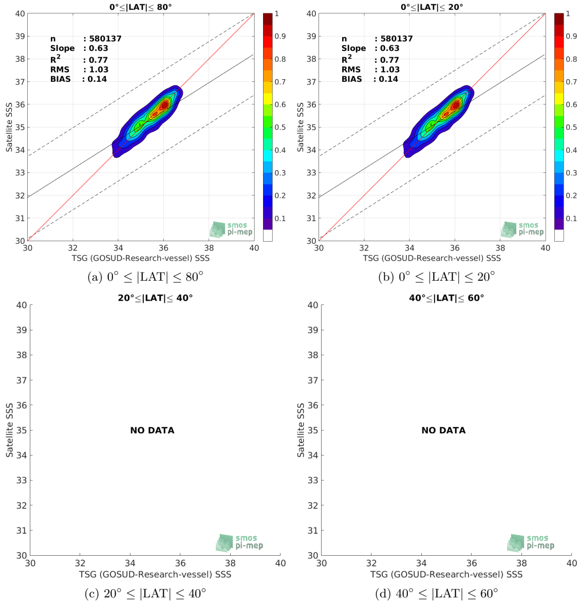
Figure 9: Contour maps of the concentration of SMOS SSS L3 v4 - 18 Days (CATDS-CECOS-LOCEAN) SSS ( y -axis) versus TSG (GOSUD-Research-vessel) SSS ( x -axis) at match-up pairs for different latitude bands. For each plot, the red line shows x=y . The black thin and dashed lines indicate a linear fit through the data cloud and the \pm 95\% confidence levels, respectively. The number match-up pairs n , the slope and R^2 coefficient of the linear fit, the root mean square (RMS) and the mean bias between satellite and in situ data are indicated for each latitude band in each plots.
