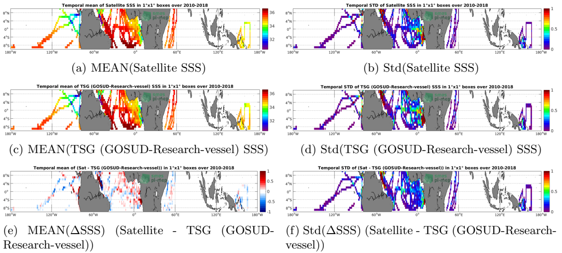
Figure 6: Temporal mean (left) and Std (right) of SSS from SMOS SSS L3 v4 - 18 Days (CATDS-CECOS-LOCEAN) (top), TSG (GOSUD-Research-vessel) (middle), and of \Delta SSS (Satellite - TSG (GOSUD-Research-vessel)). Only match-up pairs are used to generate these maps.
