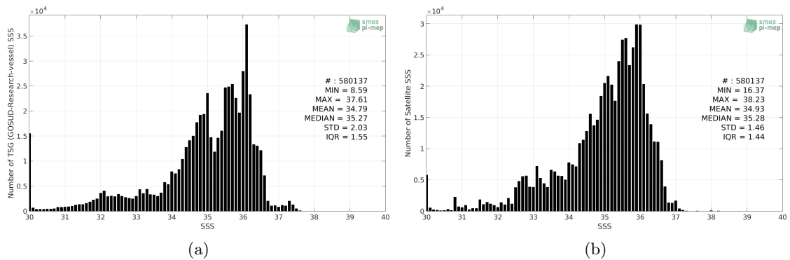
Figure 2: Histograms of SSS from TSG (GOSUD-Research-vessel) (a) and SMOS SSS L3 v4 - 18 Days (CATDS-CECOS-LOCEAN) (b) considering all match-up pairs per bins of 0.1 over the Equatorial Ocean 10N-10S Pi-MEP region and for the full satellite product period.
