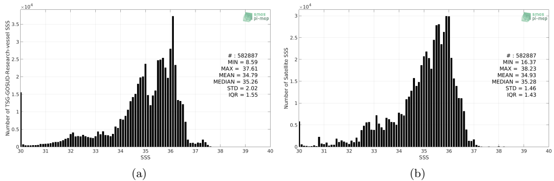
Figure 2: Histograms of SSS from TSG-GOSUD-Research-vessel (a) and SMOS-L3-CATDS-CECOS-LOCEAN-V4-18DAYS-25KM (b) considering all match-up pairs per bins of 0.1 over the Equatorial Ocean 10N-10S Pi-MEP region and for the full satellite product period.
