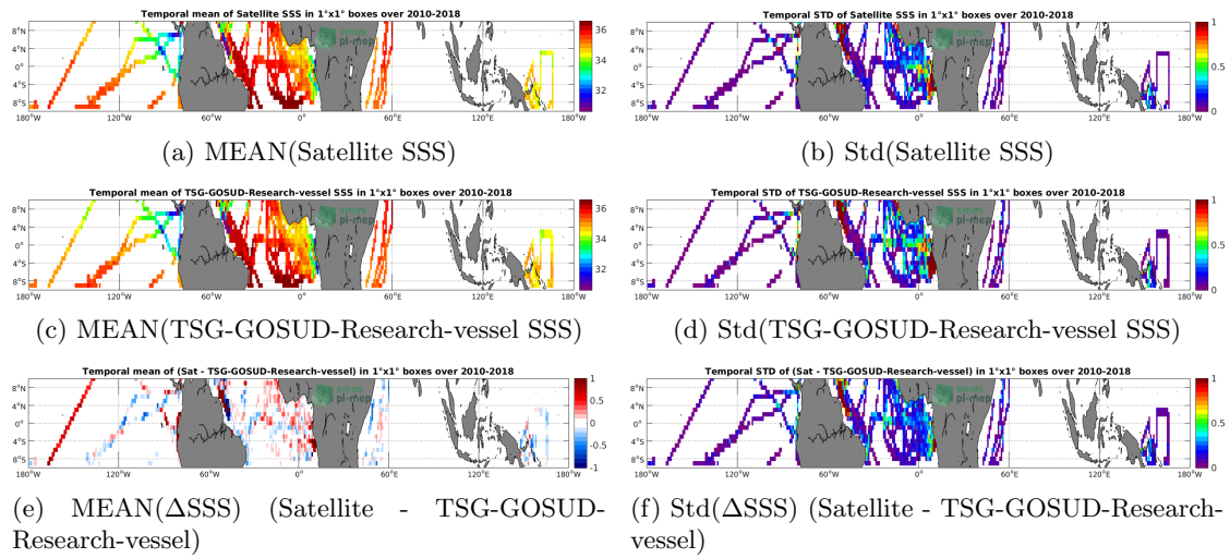
Figure 6: Temporal mean (left) and Std (right) of SSS from SMOS-L3-CATDS-CECOS-LOCEAN-V4-18DAYS-25KM (top), TSG-GOSUD-Research-vessel (middle), and of \Delta SSS (Satellite - TSG-GOSUD-Research-vessel). Only match-up pairs are used to generate these maps.
