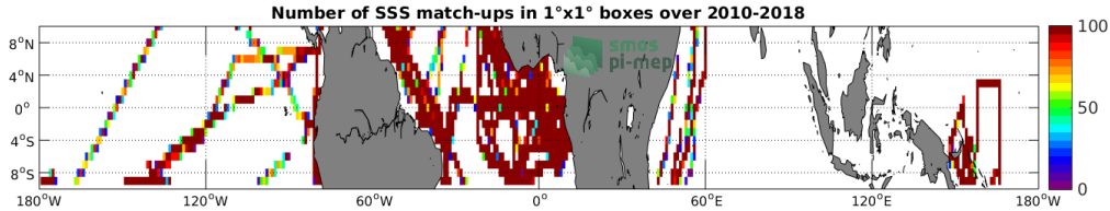
Figure 4: Number of SSS match-ups between TSG-GOSUD-Research-vessel SSS and the SMOS-L3-CATDS-CECOS-LOCEAN-V4-18DAYS-25KM SSS product for the Equatorial Ocean 10N-10S Pi-MEP region over 1°x1° boxes and for the full satellite product period.
