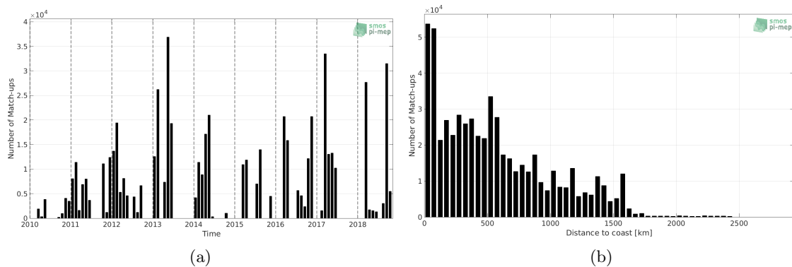
Figure 1: Number of match-ups between TSG-GOSUD-Research-vessel and SMOS-L3-CATDS-CECOS-LOCEAN-V4-18DAYS-25KM SSS as a function of time (a) and as function of the distance to coast (b) over the Equatorial Ocean 10N-10S Pi-MEP region and for the full satellite product period.
