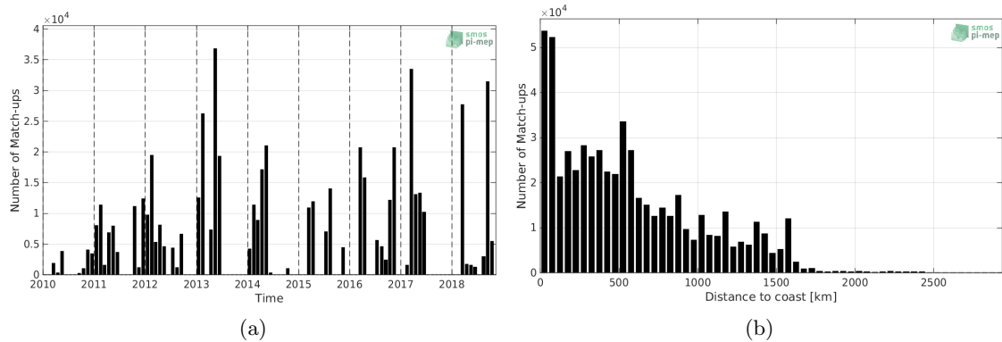
Figure 1: Number of match-ups between TSG-GOSUD-Research-vessel and SMOS-L3-CATDS-CECOS-LOCEAN-V4-18DAYS-25KM SSS as a function of time (a) and as function of the distance to coast (b) over the Equatorial Ocean 10N-10S Pi-MEP region and for the full satellite product period.
