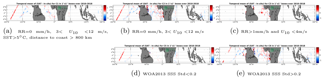
Figure 12: Temporal mean gridded over spatial boxes of size 1^\circ \times 1^\circ of \Delta SSS (SMOS-L3-CATDS-CECOS-LOCEAN-V4-18DAYS-25KM - TSG-GOSUD-Research-vessel) for 5 different subdatasets corresponding to:RR=0 mm/h, 3 < U_{10} < 12 m/s, SST >5^\circ C, distance to coast > 800 km (a), RR=0 mm/h, 3 < U_{10} < 12 m/s (b), RR >1 mm/h and U_{10} < 4 m/s (c), WOA2013 SSS Std <0.2 (d), WOA2013 SSS Std >0.2 (e).
