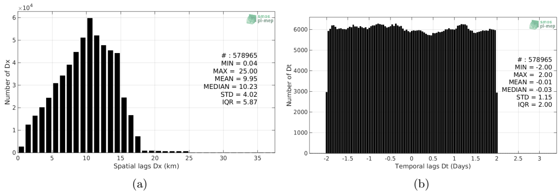
Figure 5: Histograms of the spatial (a) and temporal (b) lags between the time of the TSG-GOSUD-Research-vessel measurements and the date of the corresponding SMOS-L3-CATDS-CECOS-LOCEAN-V4-18DAYS-25KM SSS product.
