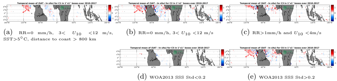
Figure 11: Temporal mean gridded over spatial boxes of size 1^\circ \times 1^\circ of \Delta SSS (SMOS-L3-CATDS-CECOS-LOCEAN-V4-18DAYS-25KM - Surface drifters) for 5 different subdatasets corresponding to:RR=0 mm/h, 3 < U_{10} < 12 m/s, SST >5^\circ C, distance to coast > 800 km (a), RR=0 mm/h, 3 < U_{10} < 12 m/s (b), RR >1 mm/h and U_{10} < 4 m/s (c), WOA2013 SSS Std <0.2 (d), WOA2013 SSS Std >0.2 (e).
