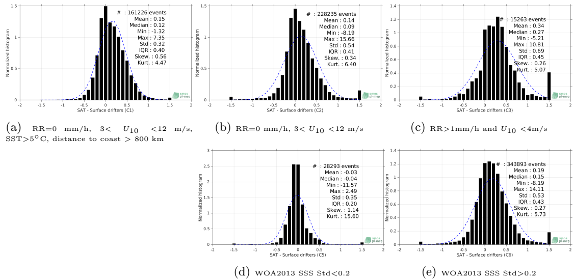
Figure 12: Normalized histogram of \Delta SSS (SMOS-L3-CATDS-CECOS-LOCEAN-V4-18DAYS-25KM - Surface drifters) for 5 different subdatasets corresponding to: RR=0 mm/h, 3 < U_{10} < 12 m/s, SST >5^\circ C, distance to coast > 800 km (a), RR=0 mm/h, 3 < U_{10} < 12 m/s (b), RR >1 mm/h and U_{10} < 4 m/s (c), WOA2013 SSS Std <0.2 (d), WOA2013 SSS Std >0.2 (e).
