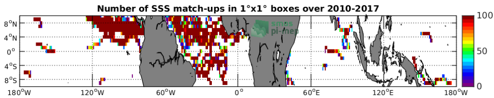
Figure 3: Number of SSS match-ups between Surface drifters SSS and the SMOS-L3-CATDS-CECOS-LOCEAN-V4-18DAYS-25KM SSS product for the Equatorial Ocean 10N-10S Pi-MEP region over 1°x1° boxes and for the full satellite product period.
