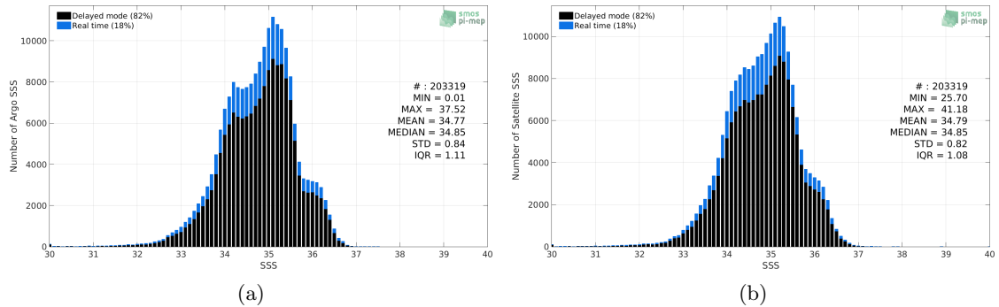
Figure 2: Histograms of SSS from Argo (a) and SMOS SSS L3 v4 - 18 Days (CATDS-CECOS-LOCEAN) (b) considering all match-up pairs per bins of 0.1 over the Equatorial Ocean 10N-10S Pi-MEP region and for the full satellite product period.
