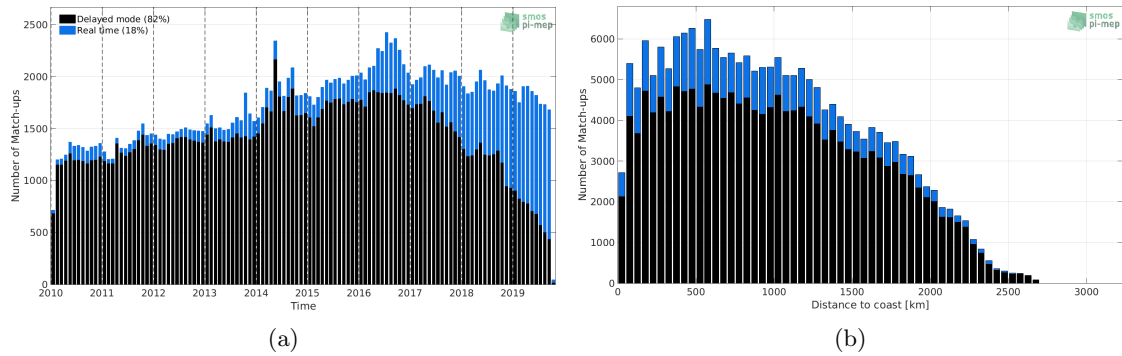
Figure 1: Number of match-ups between Argo and SMOS SSS L3 v4 - 18 Days (CATDS-CECOS-LOCEAN) SSS as a function of time (a) and as function of the distance to coast (b) over the Equatorial Ocean 10N-10S Pi-MEP region and for the full satellite product period.
