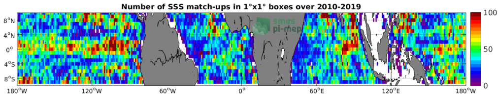
Figure 4: Number of SSS match-ups between Argo SSS and the SMOS SSS L3 v4 - 18 Days (CATDS-CECOS-LOCEAN) SSS product for the Equatorial Ocean 10N-10S Pi-MEP region over 1°x1° boxes and for the full satellite product period.
