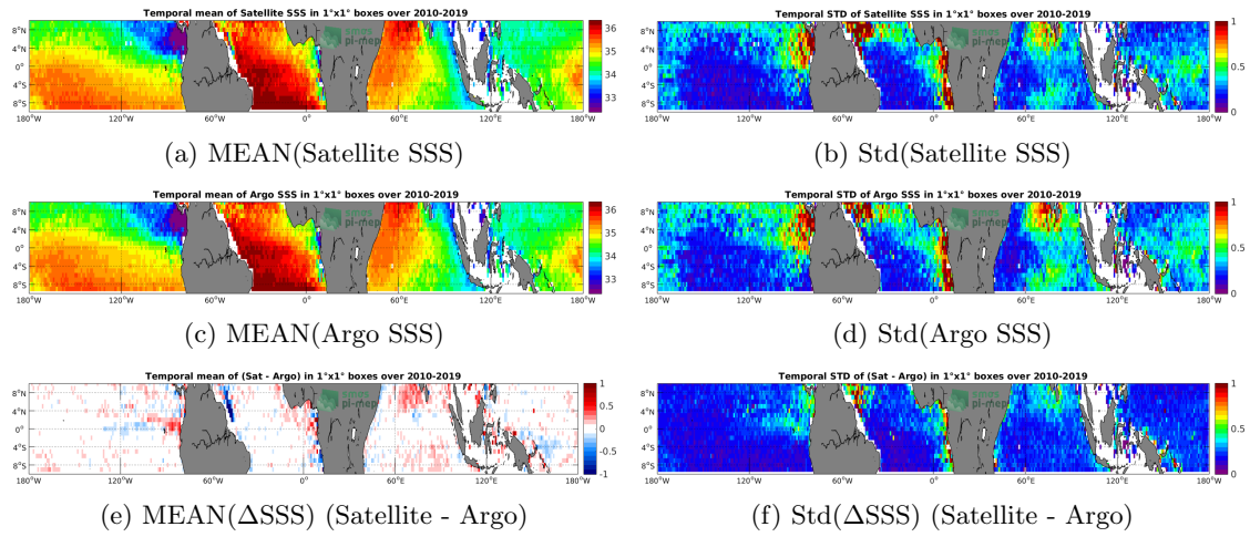
Figure 6: Temporal mean (left) and Std (right) of SSS from SMOS SSS L3 v4 - 18 Days (CATDS-CECOS-LOCEAN) (top), Argo (middle), and of \Delta SSS (Satellite - Argo). Only match-up pairs are used to generate these maps.
