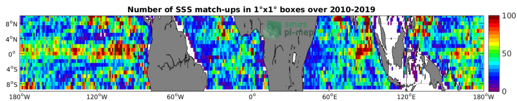
Figure 4: Number of SSS match-ups between Argo SSS and the SMOS-L3-CATDS-CECOS-LOCEAN-V4-18DAYS-25KM SSS product for the Equatorial Ocean 10N-10S Pi-MEP region over 1^\circ \times 1^\circ boxes and for the full satellite product period.
