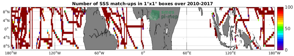
Figure 4: Number of SSS match-ups between TSG-SAMOS SSS and the SMOS-L3-CATDS-CECOS-LOCEAN-V3-9DAYS-25KM SSS product for the Equatorial Ocean 10N-10S Pi-MEP region over 1°x1° boxes and for the full satellite product period.
