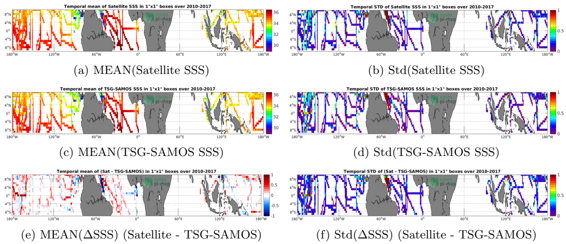
Figure 6: Temporal mean (left) and Std (right) of SSS from SMOS-L3-CATDS-CECOS-LOCEAN-V3-9DAYS-25KM (top), TSG-SAMOS (middle), and of \Delta SSS (Satellite - TSG-SAMOS). Only match-up pairs are used to generate these maps.
