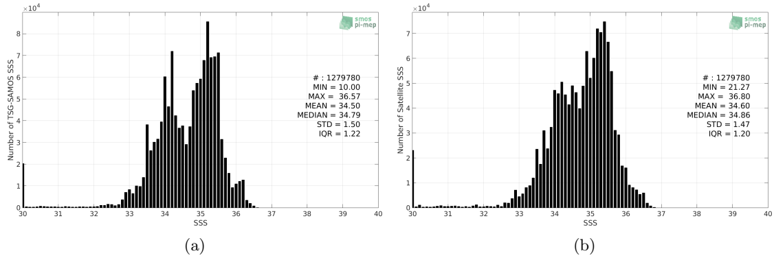
Figure 2: Histograms of SSS from TSG-SAMOS (a) and SMOS-L3-CATDS-CECOS-LOCEAN-V3-9DAYS-25KM (b) considering all match-up pairs per bins of 0.1 over the Equatorial Ocean 10N-10S Pi-MEP region and for the full satellite product period.
