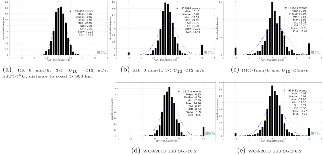
Figure 13: Normalized histogram of \Delta SSS (SMOS-L3-CATDS-CECOS-LOCEAN-V3-9DAYS-25KM - TSG-SAMOS) for 5 different subdatasets corresponding to: RR=0 mm/h, 3 < U_{10} < 12 m/s, SST > 5^\circ C , distance to coast > 800 km (a), RR=0 mm/h, 3 < U_{10} < 12 m/s (b), RR > 1 mm/h and U_{10} < 4 m/s (c), WOA2013 SSS Std < 0.2 (d), WOA2013 SSS Std > 0.2 (e).
