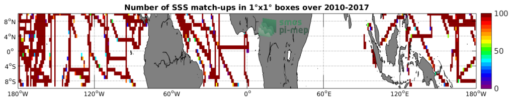
Figure 4: Number of SSS match-ups between TSG-SAMOS SSS and the SMOS-L3-CATDS-CECOS-LOCEAN-V3-9DAYS-25KM SSS product for the Equatorial Ocean 10N-10S Pi-MEP region over 1^\circ \times 1^\circ boxes and for the full satellite product period.
