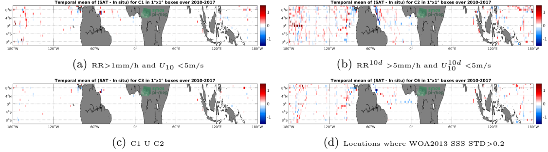
Figure 12: Temporal mean gridded over spatial boxes of size 1^\circ \times 1^\circ of \Delta SSS (SMOS-L3-CATDS-CECOS-LOCEAN-V3-9DAYS-25KM - TSG-SAMOS) for 4 different subdatasets corresponding to: RR > 1\text{mm/h} and U_{10} < 5\text{m/s} (a), RR^{10d} > 5\text{mm/h} and U_{10}^{10d} < 5\text{m/s} (b), C1 U C2 (c), Locations where WOA2013 SSS STD > 0.2 (d).
