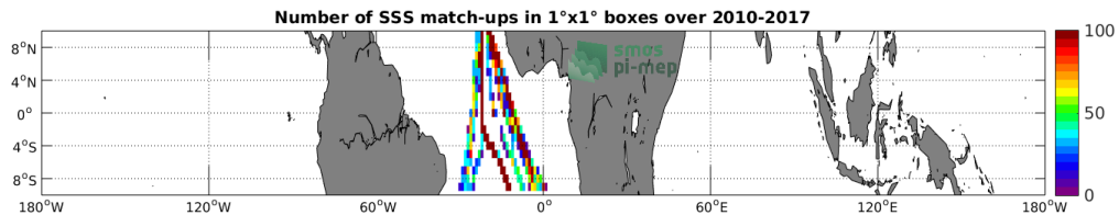
Figure 4: Number of SSS match-ups between TSG-POLARSTERN SSS and the SMOS-L3-CATDS-CECOS-LOCEAN-V3-9DAYS-25KM SSS product for the Equatorial Ocean 10N-10S Pi-MEP region over 1°x1° boxes and for the full satellite product period.
