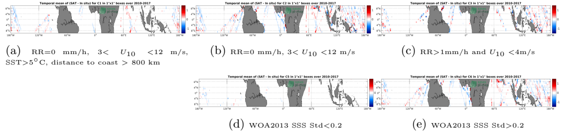
Figure 12: Temporal mean gridded over spatial boxes of size 1^\circ \times 1^\circ of \Delta SSS (SMOS-L3-CATDS-CECOS-LOCEAN-V3-9DAYS-25KM - TSG-LEGOS-DM) for 5 different subdatasets corresponding to: RR=0 mm/h, 3 < U_{10} < 12 m/s, SST > 5^\circ C , distance to coast > 800 km (a), RR=0 mm/h, 3 < U_{10} < 12 m/s (b), RR > 1 mm/h and U_{10} < 4 m/s (c), WOA2013 SSS Std < 0.2 (d), WOA2013 SSS Std > 0.2 (e).
