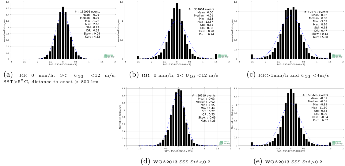
Figure 13: Normalized histogram of \Delta SSS (SMOS-L3-CATDS-CECOS-LOCEAN-V3-9DAYS-25KM - TSG-LEGOS-DM) for 5 different subdatasets corresponding to: RR=0 mm/h, 3 < U_{10} < 12 m/s, SST > 5^\circ C , distance to coast > 800 km (a), RR=0 mm/h, 3 < U_{10} < 12 m/s (b), RR > 1 mm/h and U_{10} < 4 m/s (c), WOA2013 SSS Std < 0.2 (d), WOA2013 SSS Std > 0.2 (e).
