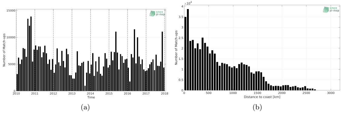
Figure 1: Number of match-ups between TSG-LEGOS-DM and SMOS-L3-CATDS-CECOS-LOCEAN-V3-9DAYS-25KM SSS as a function of time (a) and as function of the distance to coast (b) over the Equatorial Ocean 10N-10S Pi-MEP region and for the full satellite product period.
