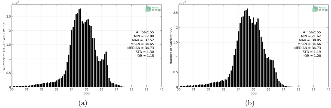
Figure 2: Histograms of SSS from TSG-LEGOS-DM (a) and SMOS-L3-CATDS-CECOS-LOCEAN-V3-9DAYS-25KM (b) considering all match-up pairs per bins of 0.1 over the Equatorial Ocean 10N-10S Pi-MEP region and for the full satellite product period.
