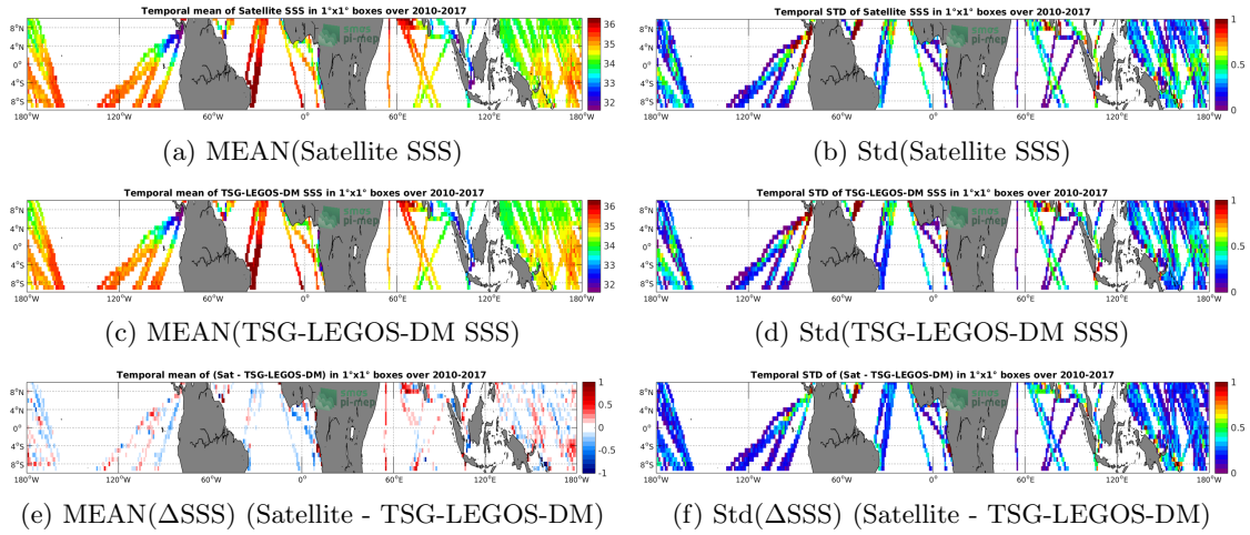
Figure 6: Temporal mean (left) and Std (right) of SSS from SMOS-L3-CATDS-CECOS-LOCEAN-V3-9DAYS-25KM (top), TSG-LEGOS-DM (middle), and of \Delta SSS (Satellite - TSG-LEGOS-DM). Only match-up pairs are used to generate these maps.
