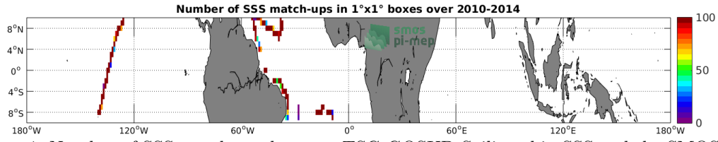
Figure 4: Number of SSS match-ups between TSG-GOSUD-Sailing-ship SSS and the SMOS-L3-CATDS-CECOS-LOCEAN-V3-9DAYS-25KM SSS product for the Equatorial Ocean 10N-10S Pi-MEP region over 1^\circ \times 1^\circ boxes and for the full satellite product period.
