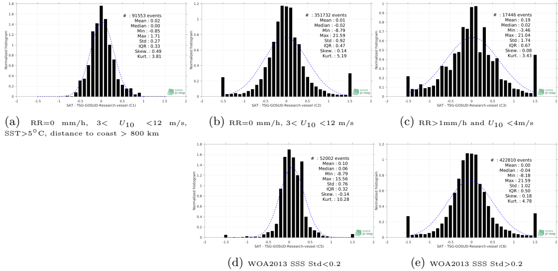
Figure 13: Normalized histogram of \Delta SSS (SMOS-L3-CATDS-CECOS-LOCEAN-V3-9DAYS-25KM - TSG-GOSUD-Research-vessel) for 5 different subdatasets corresponding to: RR=0 mm/h, 3 < U_{10} < 12 m/s, SST >5^\circ\text{C} , distance to coast > 800 km (a), RR=0 mm/h, 3 < U_{10} < 12 m/s (b), RR >1 mm/h and U_{10} < 4 m/s (c), WOA2013 SSS Std <0.2 (d), WOA2013 SSS Std >0.2 (e).
