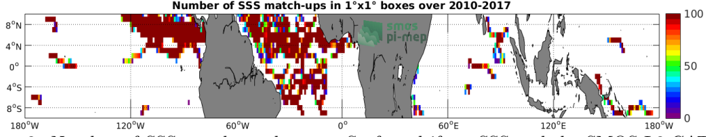
Figure 3: Number of SSS match-ups between Surface drifters SSS and the SMOS-L3-CATDS-CECOS-LOCEAN-V3-9DAYS-25KM SSS product for the Equatorial Ocean 10N-10S Pi-MEP region over 1°x1° boxes and for the full satellite product period.
