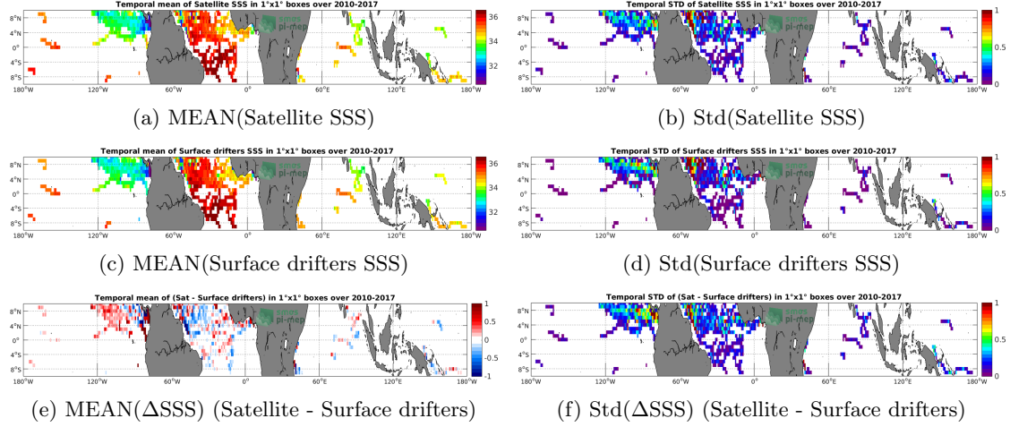
Figure 5: Temporal mean (left) and Std (right) of SSS from SMOS-L3-CATDS-CECOS-LOCEAN-V3-9DAYS-25KM (top), Surface drifters (middle), and of \Delta SSS (Satellite - Surface drifters). Only match-up pairs are used to generate these maps.
