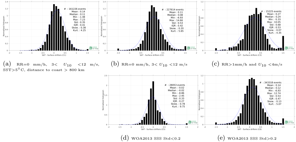
Figure 12: Normalized histogram of \Delta SSS (SMOS-L3-CATDS-CECOS-LOCEAN-V3-9DAYS-25KM - Surface drifters) for 5 different subdatasets corresponding to: RR=0 mm/h, 3 < U_{10} < 12 m/s, SST > 5^\circ C , distance to coast > 800 km (a), RR=0 mm/h, 3 < U_{10} < 12 m/s (b), RR > 1 mm/h and U_{10} < 4 m/s (c), WOA2013 SSS Std < 0.2 (d), WOA2013 SSS Std > 0.2 (e).
