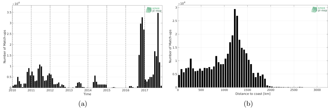
Figure 1: Number of match-ups between Surface drifters and SMOS-L3-CATDS-CECOS-LOCEAN-V3-9DAYS-25KM SSS as a function of time (a) and as function of the distance to coast (b) over the Equatorial Ocean 10N-10S Pi-MEP region and for the full satellite product period.
