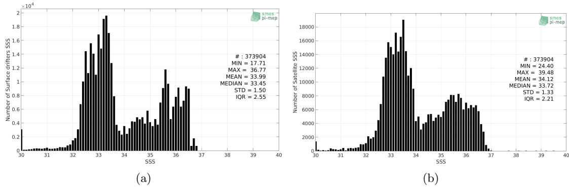
Figure 2: Histograms of SSS from Surface drifters (a) and SMOS-L3-CATDS-CECOS-LOCEAN-V3-9DAYS-25KM (b) considering all match-up pairs per bins of 0.1 over the Equatorial Ocean 10N-10S Pi-MEP region and for the full satellite product period.
