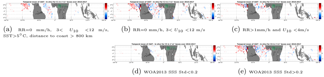
Figure 11: Temporal mean gridded over spatial boxes of size 1^\circ \times 1^\circ of \Delta SSS (SMOS-L3-CATDS-CECOS-LOCEAN-V3-9DAYS-25KM - Surface drifters) for 5 different subdatasets corresponding to: RR=0 mm/h, 3 < U_{10} < 12 m/s, SST > 5^\circ C , distance to coast > 800 km (a), RR=0 mm/h, 3 < U_{10} < 12 m/s (b), RR > 1 mm/h and U_{10} < 4 m/s (c), WOA2013 SSS Std < 0.2 (d), WOA2013 SSS Std > 0.2 (e).
