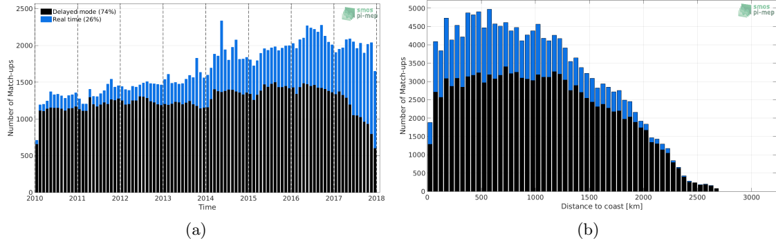
Figure 1: Number of match-ups between Argo and SMOS-L3-CATDS-CECOS-LOCEAN-V3-9DAYS-25KM SSS as a function of time (a) and as function of the distance to coast (b) over the Equatorial Ocean 10N-10S Pi-MEP region and for the full satellite product period.
