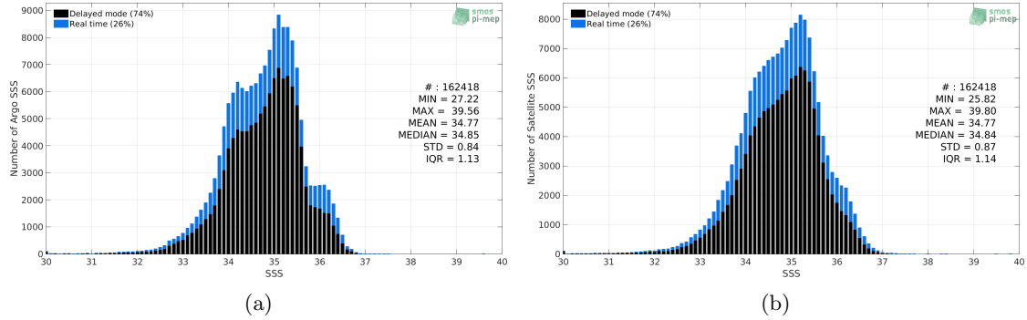
Figure 2: Histograms of SSS from Argo (a) and SMOS-L3-CATDS-CECOS-LOCEAN-V3-9DAYS-25KM (b) considering all match-up pairs per bins of 0.1 over the Equatorial Ocean 10N-10S Pi-MEP region and for the full satellite product period.
