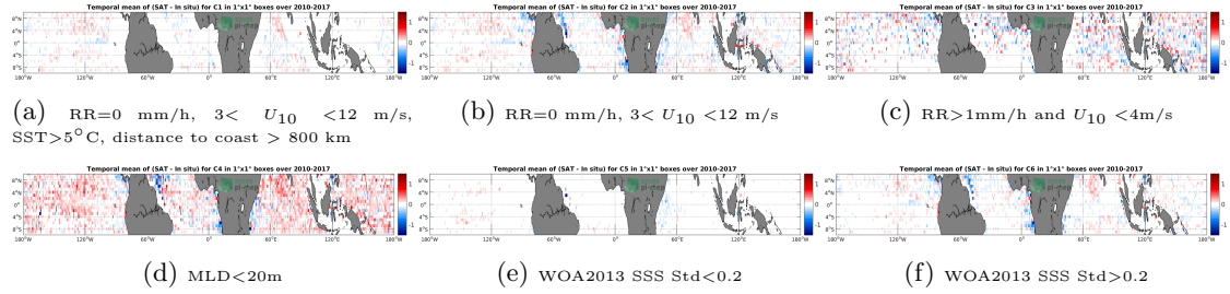
Figure 12: Temporal mean gridded over spatial boxes of size 1^\circ \times 1^\circ of \Delta SSS (SMOS-L3-CATDS-CECOS-LOCEAN-V3-9DAYS-25KM - Argo) for 6 different subdatasets corresponding to: RR=0 mm/h, 3 < U_{10} < 12 m/s, SST > 5^\circ C , distance to coast > 800 km (a), RR=0 mm/h, 3 < U_{10} < 12 m/s (b), RR > 1 mm/h and U_{10} < 4 m/s (c), MLD < 20 m (d), WOA2013 SSS Std < 0.2 (e), WOA2013 SSS Std > 0.2 (f).
