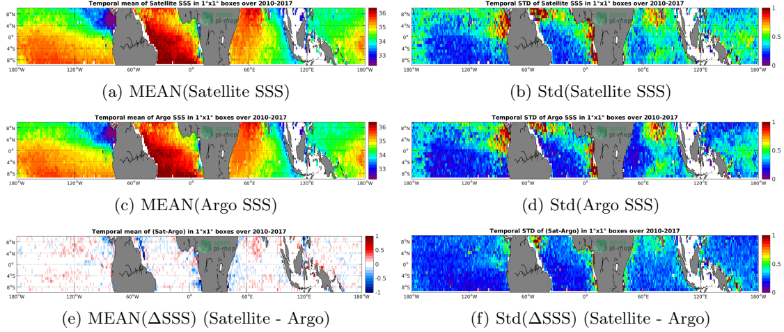
Figure 6: Temporal mean (left) and Std (right) of SSS from SMOS-L3-CATDS-CECOS-LOCEAN-V3-9DAYS-25KM (top), Argo (middle), and of \Delta SSS (Satellite - Argo). Only match-up pairs are used to generate these maps.
