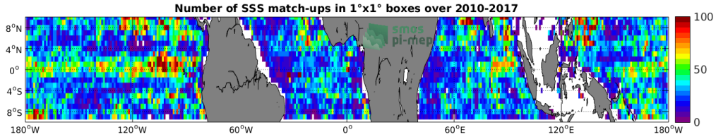
Figure 4: Number of SSS match-ups between Argo SSS and the SMOS-L3-CATDS-CECOS-LOCEAN-V3-9DAYS-25KM SSS product for the Equatorial Ocean 10N-10S Pi-MEP region over 1^\circ \times 1^\circ boxes and for the full satellite product period.
