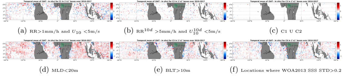
Figure 12: Temporal mean gridded over spatial boxes of size 1^\circ \times 1^\circ of \Delta\text{SSS} (SMOS-L3-CATDS-CECOS-LOCEAN-V3-9DAYS-25KM - Argo) for 6 different subdatasets corresponding to: \text{RR} > 1\text{mm/h} and U_{10} < 5\text{m/s} (a), \text{RR}^{10d} > 5\text{mm/h} and U_{10}^{10d} < 5\text{m/s} (b), C1 U C2 (c), \text{MLD} < 20\text{m} (d), \text{BLT} > 10\text{m} (e), Locations where WOA2013 SSS STD > 0.2 (f).
