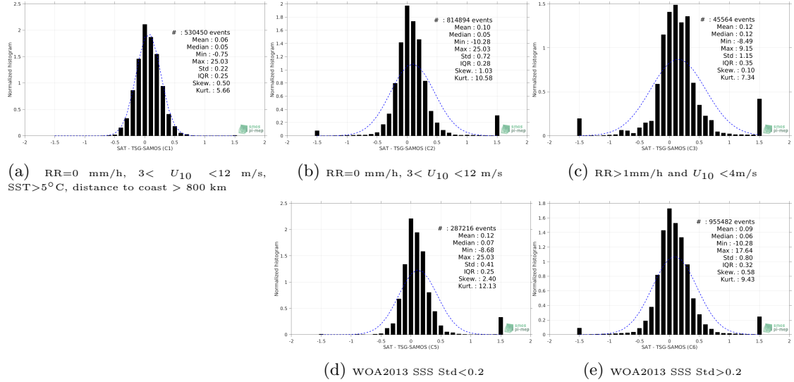
Figure 13: Normalized histogram of \Delta SSS (SMOS-L3-CATDS-CECOS-LOCEAN-V3-18DAYS-25KM - TSG-SAMOS) for 5 different subdatasets corresponding to: RR=0 mm/h, 3 < U_{10} < 12 m/s, SST > 5^\circ C , distance to coast > 800 km (a), RR=0 mm/h, 3 < U_{10} < 12 m/s (b), RR > 1 mm/h and U_{10} < 4 m/s (c), WOA2013 SSS Std < 0.2 (d), WOA2013 SSS Std > 0.2 (e).
