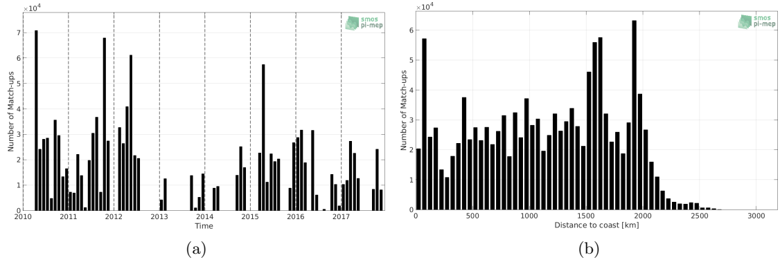
Figure 1: Number of match-ups between TSG-SAMOS and SMOS-L3-CATDS-CECOS-LOCEAN-V3-18DAYS-25KM SSS as a function of time (a) and as function of the distance to coast (b) over the Equatorial Ocean 10N-10S Pi-MEP region and for the full satellite product period.
