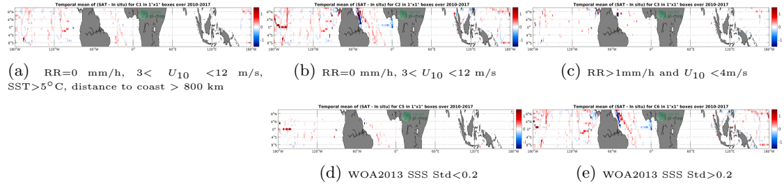
Figure 12: Temporal mean gridded over spatial boxes of size 1^\circ \times 1^\circ of \Delta SSS (SMOS-L3-CATDS-CECOS-LOCEAN-V3-18DAYS-25KM - TSG-SAMOS) for 5 different subdatasets corresponding to: RR=0 mm/h, 3 < U_{10} < 12 m/s, SST > 5^\circ C , distance to coast > 800 km (a), RR=0 mm/h, 3 < U_{10} < 12 m/s (b), RR > 1 mm/h and U_{10} < 4 m/s (c), WOA2013 SSS Std < 0.2 (d), WOA2013 SSS Std > 0.2 (e).
