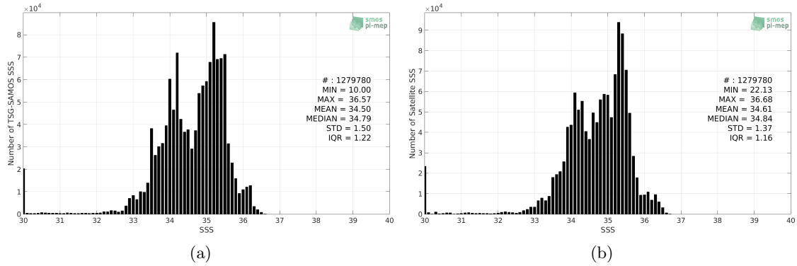
Figure 2: Histograms of SSS from TSG-SAMOS (a) and SMOS-L3-CATDS-CECOS-LOCEAN-V3-18DAYS-25KM (b) considering all match-up pairs per bins of 0.1 over the Equatorial Ocean 10N-10S Pi-MEP region and for the full satellite product period.
