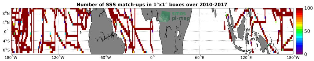
Figure 4: Number of SSS match-ups between TSG-SAMOS SSS and the SMOS-L3-CATDS-CECOS-LOCEAN-V3-18DAYS-25KM SSS product for the Equatorial Ocean 10N-10S Pi-MEP region over 1°x1° boxes and for the full satellite product period.
