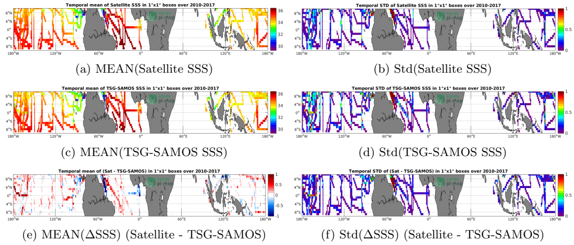
Figure 6: Temporal mean (left) and Std (right) of SSS from SMOS-L3-CATDS-CECOS-LOCEAN-V3-18DAYS-25KM (top), TSG-SAMOS (middle), and of \Delta SSS (Satellite - TSG-SAMOS). Only match-up pairs are used to generate these maps.
