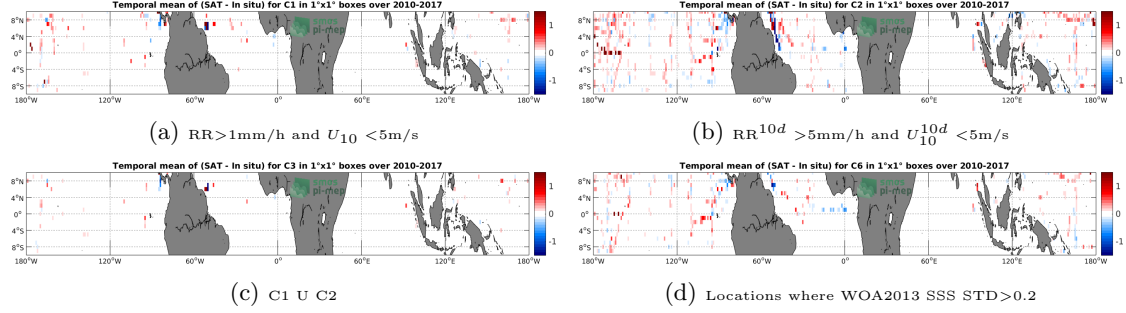
Figure 12: Temporal mean gridded over spatial boxes of size 1^\circ \times 1^\circ of \Delta SSS (SMOS-L3-CATDS-CECOS-LOCEAN-V3-18DAYS-25KM - TSG-SAMOS) for 4 different subdatasets corresponding to: RR > 1\text{mm/h} and U_{10} < 5\text{m/s} (a), RR^{10d} > 5\text{mm/h} and U_{10}^{10d} < 5\text{m/s} (b), C1 U C2 (c), Locations where WOA2013 SSS STD > 0.2 (d).
