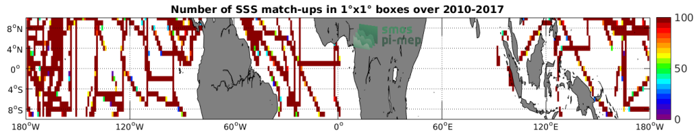
Figure 4: Number of SSS match-ups between TSG-SAMOS SSS and the SMOS-L3-CATDS-CECOS-LOCEAN-V3-18DAYS-25KM SSS product for the Equatorial Ocean 10N-10S Pi-MEP region over 1^\circ \times 1^\circ boxes and for the full satellite product period.
