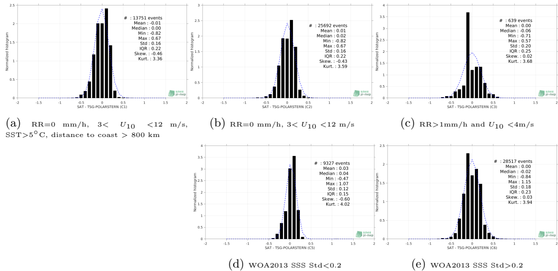
Figure 13: Normalized histogram of \Delta SSS (SMOS-L3-CATDS-CECOS-LOCEAN-V3-18DAYS-25KM - TSG-POLARSTERN) for 5 different subdatasets corresponding to: RR=0 mm/h, 3 < U_{10} < 12 m/s, SST >5^\circ C, distance to coast > 800 km (a), RR=0 mm/h, 3 < U_{10} < 12 m/s (b), RR >1 mm/h and U_{10} < 4 m/s (c), WOA2013 SSS Std <0.2 (d), WOA2013 SSS Std >0.2 (e).
