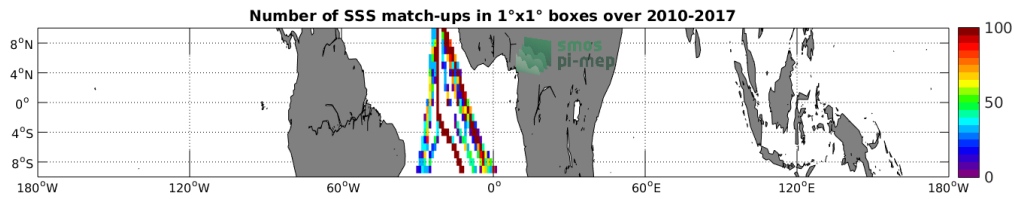
Figure 4: Number of SSS match-ups between TSG-POLARSTERN SSS and the SMOS-L3-CATDS-CECOS-LOCEAN-V3-18DAYS-25KM SSS product for the Equatorial Ocean 10N-10S Pi-MEP region over 1°x1° boxes and for the full satellite product period.
