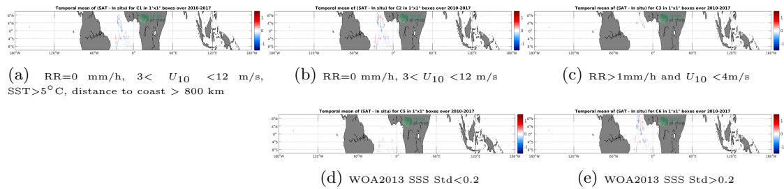
Figure 12: Temporal mean gridded over spatial boxes of size 1^\circ \times 1^\circ of \Delta SSS (SMOS-L3-CATDS-CECOS-LOCEAN-V3-18DAYS-25KM - TSG-POLARSTERN) for 5 different subdatasets corresponding to:RR=0 mm/h, 3 < U_{10} < 12 m/s, SST >5^\circ C, distance to coast > 800 km (a), RR=0 mm/h, 3 < U_{10} < 12 m/s (b), RR >1 mm/h and U_{10} < 4 m/s (c), WOA2013 SSS Std <0.2 (d), WOA2013 SSS Std >0.2 (e).
