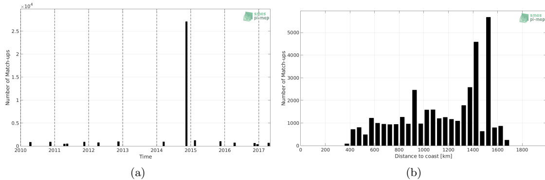
Figure 1: Number of match-ups between TSG-POLARSTERN and SMOS-L3-CATDS-CECOS-LOCEAN-V3-18DAYS-25KM SSS as a function of time (a) and as function of the distance to coast (b) over the Equatorial Ocean 10N-10S Pi-MEP region and for the full satellite product period.
