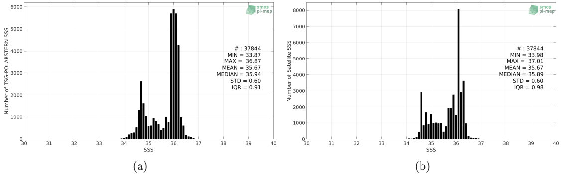
Figure 2: Histograms of SSS from TSG-POLARSTERN (a) and SMOS-L3-CATDS-CECOS-LOCEAN-V3-18DAYS-25KM (b) considering all match-up pairs per bins of 0.1 over the Equatorial Ocean 10N-10S Pi-MEP region and for the full satellite product period.
