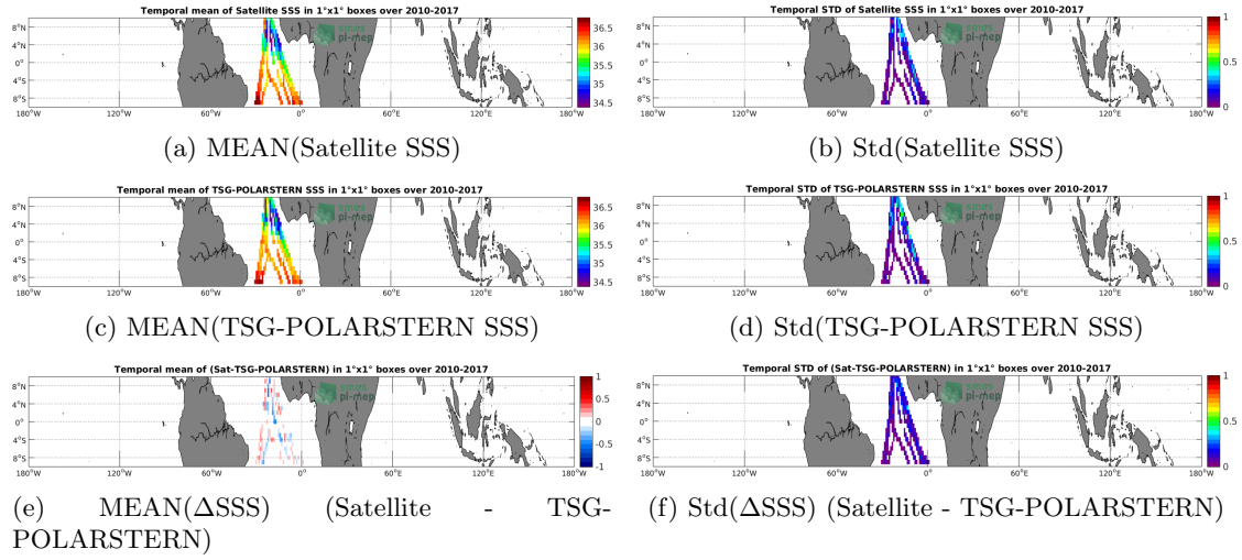
Figure 6: Temporal mean (left) and Std (right) of SSS from SMOS-L3-CATDS-CECOS-LOCEAN-V3-18DAYS-25KM (top), TSG-POLARSTERN (middle), and of \Delta SSS (Satellite - TSG-POLARSTERN). Only match-up pairs are used to generate these maps.
