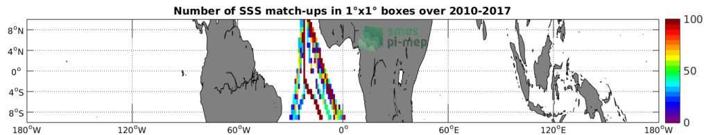
Figure 4: Number of SSS match-ups between TSG-POLARSTERN SSS and the SMOS-L3-CATDS-CECOS-LOCEAN-V3-18DAYS-25KM SSS product for the Equatorial Ocean 10N-10S Pi-MEP region over 1^\circ \times 1^\circ boxes and for the full satellite product period.
