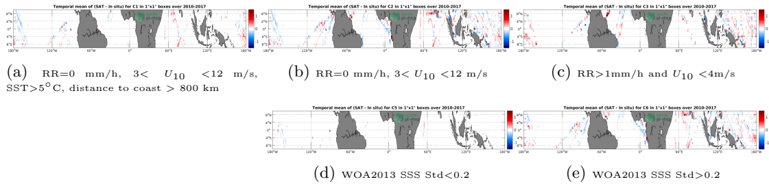
Figure 12: Temporal mean gridded over spatial boxes of size 1°x1° of ΔSSS (SMOS-L3-CATDS-CECOS-LOCEAN-V3-18DAYS-25KM - TSG-LEGOS-DM) for 5 different subdatasets corresponding to:RR=0 mm/h, 3 < U 10 < 12 m/s, SST>5°C, distance to coast > 800 km (a), RR=0 mm/h, 3 < U 10 < 12 m/s (b), RR>1mm/h and U 10 < 4m/s (c), WOA2013 SSS Std<0.2 (d), WOA2013 SSS Std>0.2 (e).
