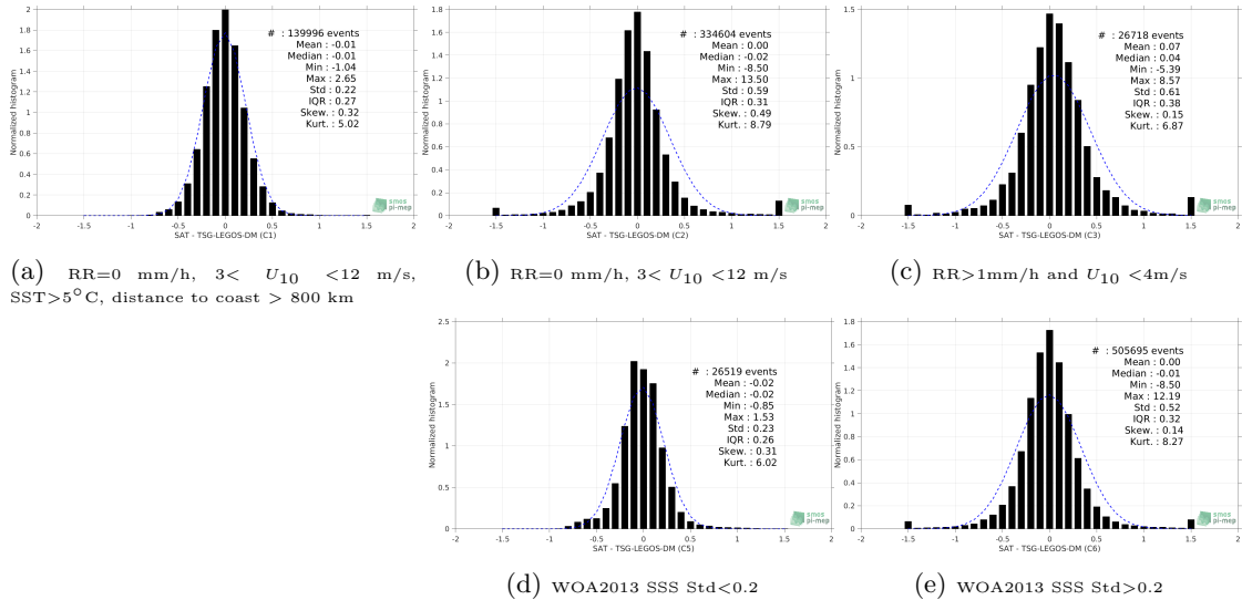
Figure 13: Normalized histogram of ΔSSS (SMOS-L3-CATDS-CECOS-LOCEAN-V3-18DAYS-25KM - TSG-LEGOS-DM) for 5 different subdatasets corresponding to: RR=0 mm/h, 3 < U 10 < 12 m/s, SST>5°C, distance to coast > 800 km (a), RR=0 mm/h, 3 < U 10 < 12 m/s (b), RR>1mm/h and U 10 < 4m/s (c), WOA2013 SSS Std<0.2 (d), WOA2013 SSS Std>0.2 (e).
