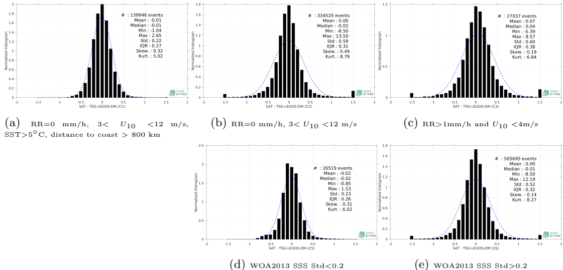
Figure 13: Normalized histogram of \Delta SSS (SMOS-L3-CATDS-CECOS-LOCEAN-V3-18DAYS-25KM - TSG-LEGOS-DM) for 5 different subdatasets corresponding to: RR=0 mm/h, 3 < U_{10} < 12 m/s, SST >5^\circ C, distance to coast > 800 km (a), RR=0 mm/h, 3 < U_{10} < 12 m/s (b), RR >1 mm/h and U_{10} < 4 m/s (c), WOA2013 SSS Std <0.2 (d), WOA2013 SSS Std >0.2 (e).
