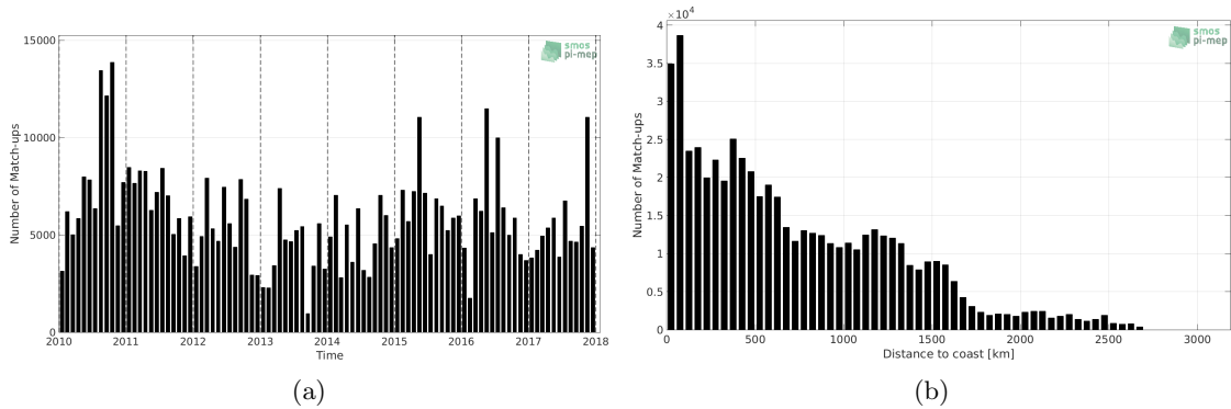
Figure 1: Number of match-ups between TSG-LEGOS-DM and SMOS-L3-CATDS-CECOS-LOCEAN-V3-18DAYS-25KM SSS as a function of time (a) and as function of the distance to coast (b) over the Equatorial Ocean 10N-10S Pi-MEP region and for the full satellite product period.
