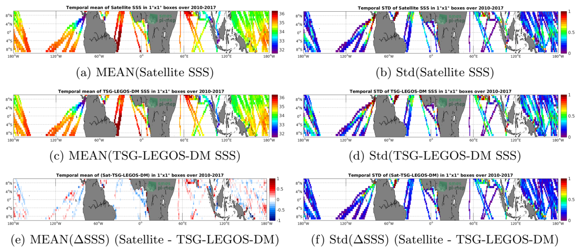
Figure 6: Temporal mean (left) and Std (right) of SSS from SMOS-L3-CATDS-CECOS-LOCEAN-V3-18DAYS-25KM (top), TSG-LEGOS-DM (middle), and of \Delta SSS (Satellite - TSG-LEGOS-DM). Only match-up pairs are used to generate these maps.
