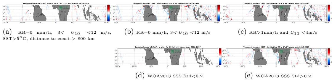
Figure 12: Temporal mean gridded over spatial boxes of size 1^\circ \times 1^\circ of \Delta SSS (SMOS-L3-CATDS-CECOS-LOCEAN-V3-18DAYS-25KM - TSG-LEGOS-DM) for 5 different subdatasets corresponding to:RR=0 mm/h, 3 < U_{10} < 12 m/s, SST >5^\circ C, distance to coast > 800 km (a), RR=0 mm/h, 3 < U_{10} < 12 m/s (b), RR >1 mm/h and U_{10} < 4 m/s (c), WOA2013 SSS Std <0.2 (d), WOA2013 SSS Std >0.2 (e).
