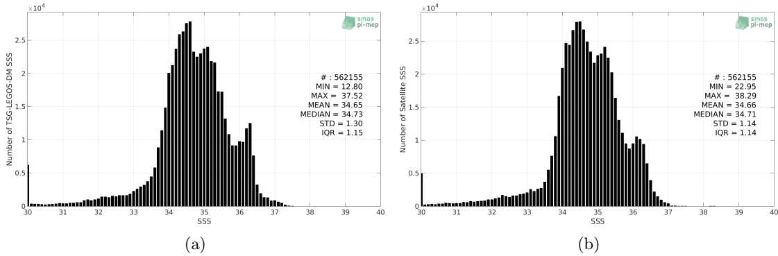
Figure 2: Histograms of SSS from TSG-LEGOS-DM (a) and SMOS-L3-CATDS-CECOS-LOCEAN-V3-18DAYS-25KM (b) considering all match-up pairs per bins of 0.1 over the Equatorial Ocean 10N-10S Pi-MEP region and for the full satellite product period.
