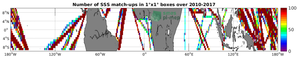
Figure 4: Number of SSS match-ups between TSG-LEGOS-DM SSS and the SMOS-L3-CATDS-CECOS-LOCEAN-V3-18DAYS-25KM SSS product for the Equatorial Ocean 10N-10S Pi-MEP region over 1^\circ \times 1^\circ boxes and for the full satellite product period.
