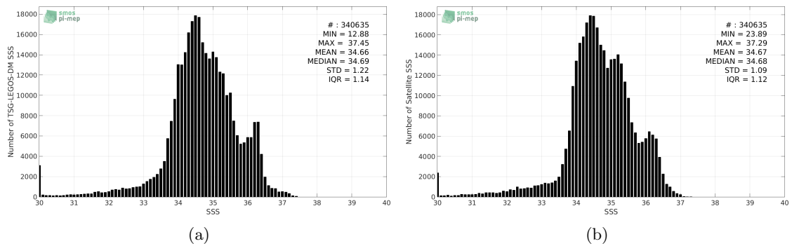
Figure 2: Histograms of SSS from TSG-LEGOS-DM (a) and SMOS-L3-CATDS-CECOS-LOCEAN-V3-18DAYS-25KM (b) considering all match-up pairs per bins of 0.1 over the Equatorial Ocean 10N-10S Pi-MEP region and for the full satellite product period.
