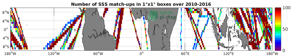
Figure 4: Number of SSS match-ups between TSG-LEGOS-DM SSS and the SMOS-L3-CATDS-CECOS-LOCEAN-V3-18DAYS-25KM SSS product for the Equatorial Ocean 10N-10S Pi-MEP region over 1°x1° boxes and for the full satellite product period.
