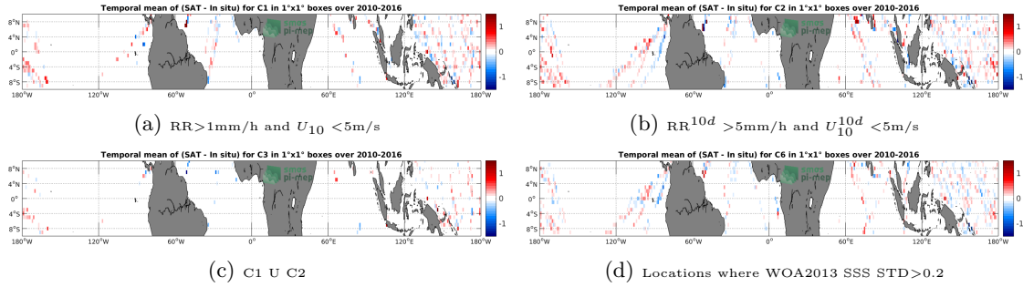
Figure 12: Temporal mean gridded over spatial boxes of size 1^\circ \times 1^\circ of \Delta SSS (SMOS-L3-CATDS-CECOS-LOCEAN-V3-18DAYS-25KM - TSG-LEGOS-DM) for 4 different subdatasets corresponding to: RR>1mm/h and U_{10} < 5\text{m/s} (a), RR^{10d} > 5\text{mm/h} and U_{10}^{10d} < 5\text{m/s} (b), C1 U C2 (c), Locations where WOA2013 SSS STD>0.2 (d).
