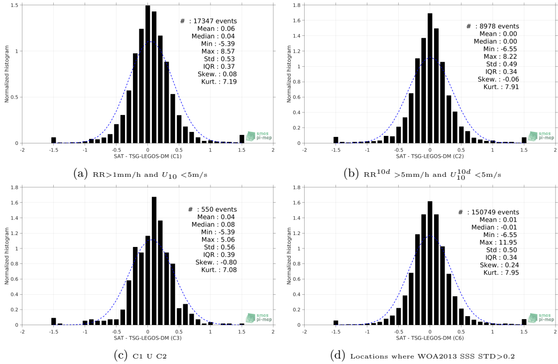
Figure 13: Normalized histogram of \Delta SSS (SMOS-L3-CATDS-CECOS-LOCEAN-V3-18DAYS-25KM - TSG-LEGOS-DM) for 6 different subdatasets corresponding to: RR>1mm/h and U_{10} < 5\text{m/s} (a), RR^{10d} > 5\text{mm/h} and U_{10}^{10d} < 5\text{m/s} (b), C1 U C2 (c), Locations where WOA2013 SSS STD>0.2 (d).
