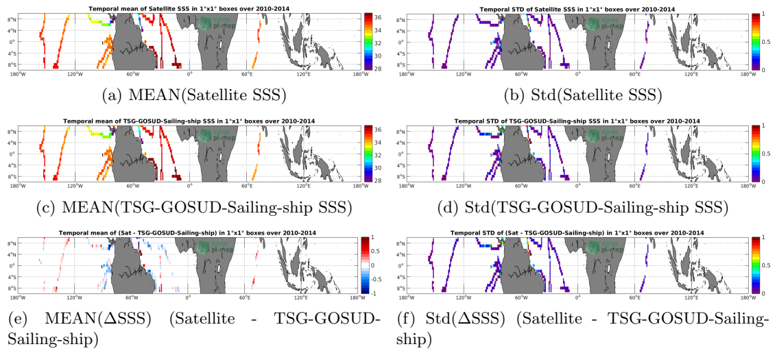
Figure 6: Temporal mean (left) and Std (right) of SSS from SMOS-L3-CATDS-CECOS-LOCEAN-V3-18DAYS-25KM (top), TSG-GOSUD-Sailing-ship (middle), and of \Delta SSS (Satellite - TSG-GOSUD-Sailing-ship). Only match-up pairs are used to generate these maps.
