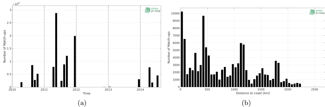
Figure 1: Number of match-ups between TSG-GOSUD-Sailing-ship and SMOS-L3-CATDS-CECOS-LOCEAN-V3-18DAYS-25KM SSS as a function of time (a) and as function of the distance to coast (b) over the Equatorial Ocean 10N-10S Pi-MEP region and for the full satellite product period.
