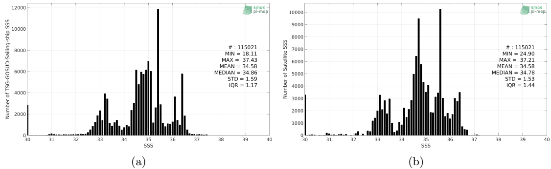
Figure 2: Histograms of SSS from TSG-GOSUD-Sailing-ship (a) and SMOS-L3-CATDS-CECOS-LOCEAN-V3-18DAYS-25KM (b) considering all match-up pairs per bins of 0.1 over the Equatorial Ocean 10N-10S Pi-MEP region and for the full satellite product period.
