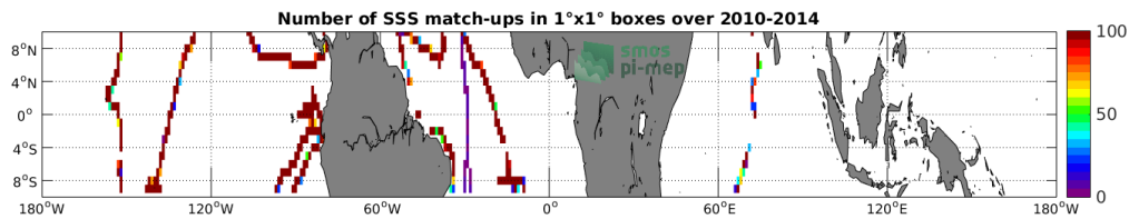
Figure 4: Number of SSS match-ups between TSG-GOSUD-Sailing-ship SSS and the SMOS-L3-CATDS-CECOS-LOCEAN-V3-18DAYS-25KM SSS product for the Equatorial Ocean 10N-10S Pi-MEP region over 1^\circ \times 1^\circ boxes and for the full satellite product period.
