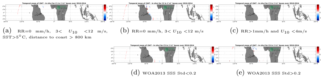
Figure 12: Temporal mean gridded over spatial boxes of size 1^\circ \times 1^\circ of \Delta SSS (SMOS-L3-CATDS-CECOS-LOCEAN-V3-18DAYS-25KM - TSG-GOSUD-Sailing-ship) for 5 different subdatasets corresponding to:RR=0 mm/h, 3 < U_{10} < 12 m/s, SST >5^\circ C, distance to coast > 800 km (a), RR=0 mm/h, 3 < U_{10} < 12 m/s (b), RR >1 mm/h and U_{10} < 4 m/s (c), WOA2013 SSS Std <0.2 (d), WOA2013 SSS Std >0.2 (e).
