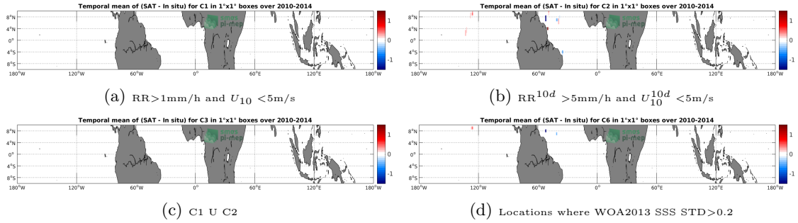
Figure 12: Temporal mean gridded over spatial boxes of size 1°x1° of ΔSSS (SMOS-L3-CATDS-CECOS-LOCEAN-V3-18DAYS-25KM - TSG-GOSUD-Sailing-ship) for 4 different subdatasets corresponding to: RR>1mm/h and U_{10} < 5\text{m/s} (a), RR^{10d} > 5\text{mm/h} and U_{10}^{10d} < 5\text{m/s} (b), C1 U C2 (c), Locations where WOA2013 SSS STD>0.2 (d).
