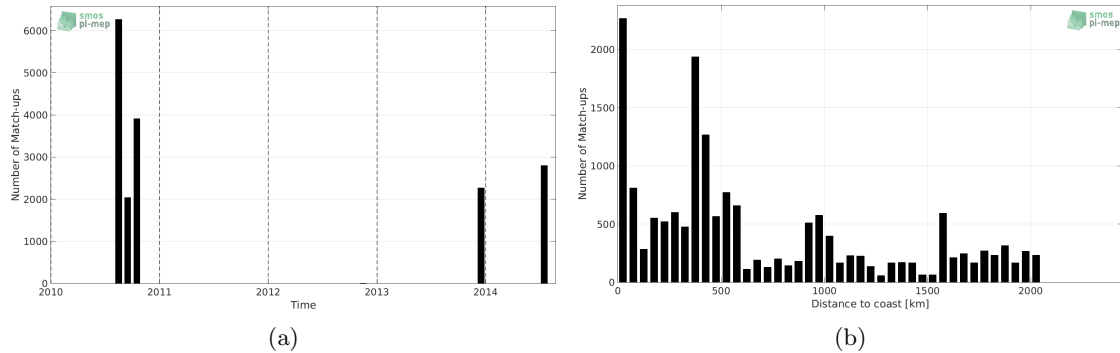
Figure 1: Number of match-ups between TSG-GOSUD-Sailing-ship and SMOS-L3-CATDS-CECOS-LOCEAN-V3-18DAYS-25KM SSS as a function of time (a) and as function of the distance to coast (b) over the Equatorial Ocean 10N-10S Pi-MEP region and for the full satellite product period.
