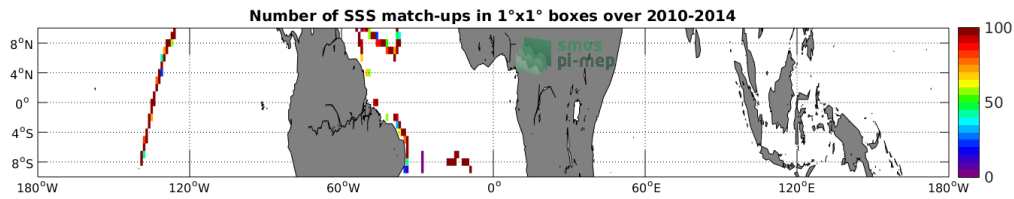
Figure 4: Number of SSS match-ups between TSG-GOSUD-Sailing-ship SSS and the SMOS-L3-CATDS-CECOS-LOCEAN-V3-18DAYS-25KM SSS product for the Equatorial Ocean 10N-10S Pi-MEP region over 1°x1° boxes and for the full satellite product period.
