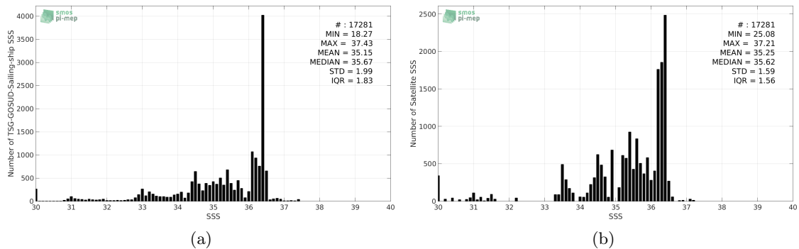
Figure 2: Histograms of SSS from TSG-GOSUD-Sailing-ship (a) and SMOS-L3-CATDS-CECOS-LOCEAN-V3-18DAYS-25KM (b) considering all match-up pairs per bins of 0.1 over the Equatorial Ocean 10N-10S Pi-MEP region and for the full satellite product period.
