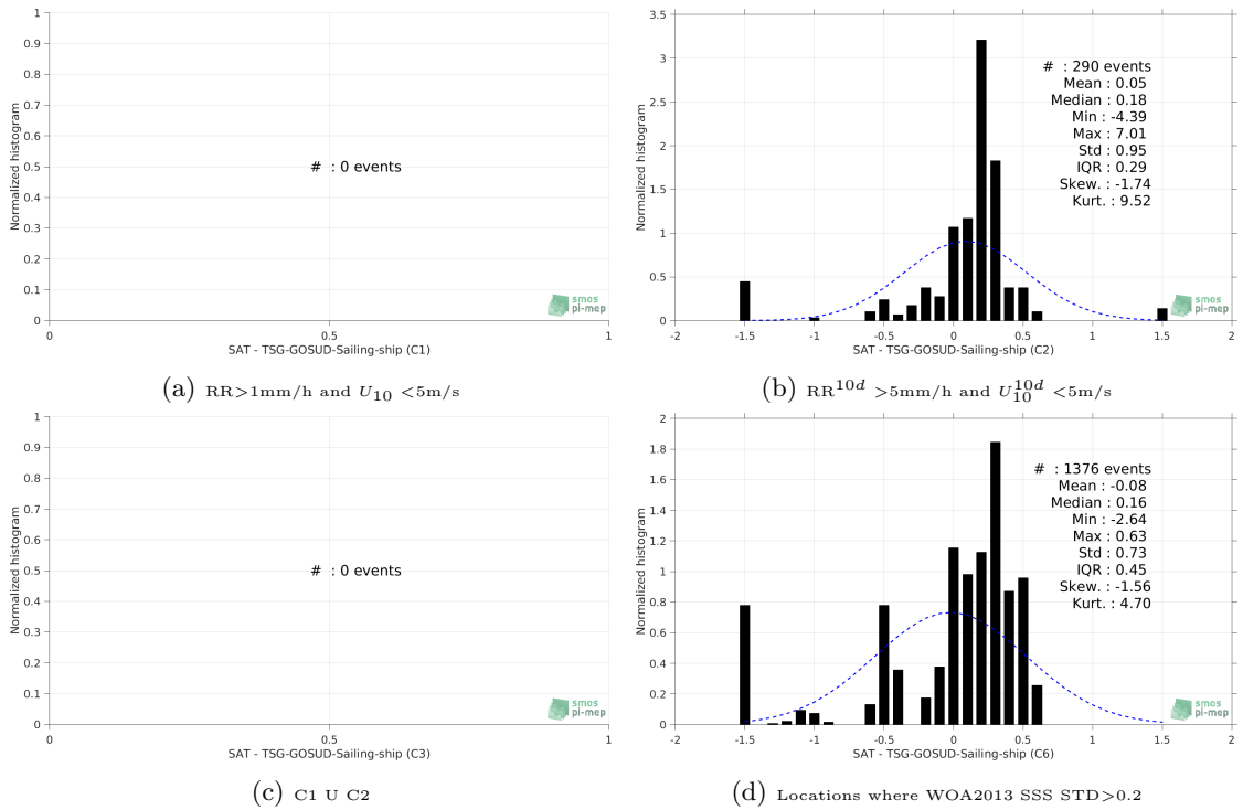
Figure 13: Normalized histogram of ΔSSS (SMOS-L3-CATDS-CECOS-LOCEAN-V3-18DAYS-25KM - TSG-GOSUD-Sailing-ship) for 6 different subdatasets corresponding to: RR>1mm/h and U_{10} < 5\text{m/s} (a), RR^{10d} > 5\text{mm/h} and U_{10}^{10d} < 5\text{m/s} (b), C1 U C2 (c), Locations where WOA2013 SSS STD>0.2 (d).
