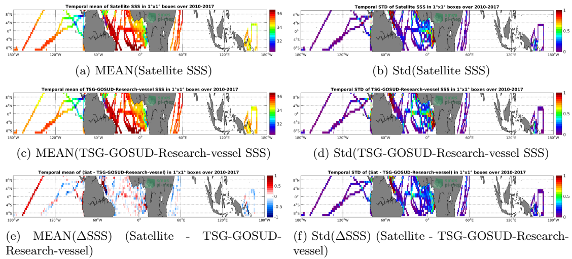
Figure 6: Temporal mean (left) and Std (right) of SSS from SMOS-L3-CATDS-CECOS-LOCEAN-V3-18DAYS-25KM (top), TSG-GOSUD-Research-vessel (middle), and of \Delta SSS (Satellite - TSG-GOSUD-Research-vessel). Only match-up pairs are used to generate these maps.
