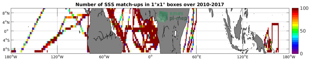
Figure 4: Number of SSS match-ups between TSG-GOSUD-Research-vessel SSS and the SMOS-L3-CATDS-CECOS-LOCEAN-V3-18DAYS-25KM SSS product for the Equatorial Ocean 10N-10S Pi-MEP region over 1°x1° boxes and for the full satellite product period.
