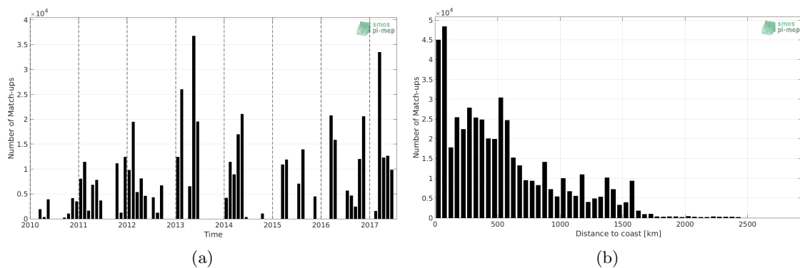
Figure 1: Number of match-ups between TSG-GOSUD-Research-vessel and SMOS-L3-CATDS-CECOS-LOCEAN-V3-18DAYS-25KM SSS as a function of time (a) and as function of the distance to coast (b) over the Equatorial Ocean 10N-10S Pi-MEP region and for the full satellite product period.
