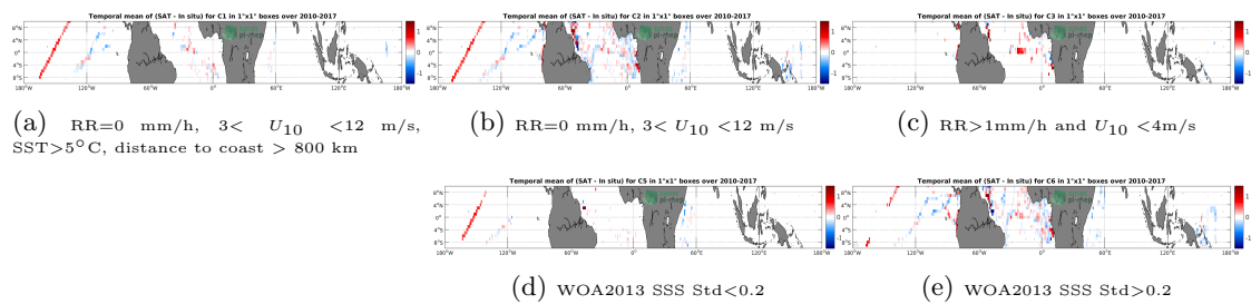
Figure 12: Temporal mean gridded over spatial boxes of size 1^\circ \times 1^\circ of \Delta SSS (SMOS-L3-CATDS-CECOS-LOCEAN-V3-18DAYS-25KM - TSG-GOSUD-Research-vessel) for 5 different subdatasets corresponding to:RR=0 mm/h, 3 < U_{10} < 12 m/s, SST >5^\circ C, distance to coast > 800 km (a), RR=0 mm/h, 3 < U_{10} < 12 m/s (b), RR >1 mm/h and U_{10} < 4 m/s (c), WOA2013 SSS Std <0.2 (d), WOA2013 SSS Std >0.2 (e).
