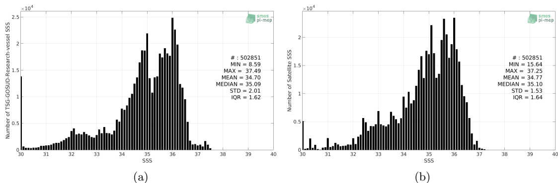
Figure 2: Histograms of SSS from TSG-GOSUD-Research-vessel (a) and SMOS-L3-CATDS-CECOS-LOCEAN-V3-18DAYS-25KM (b) considering all match-up pairs per bins of 0.1 over the Equatorial Ocean 10N-10S Pi-MEP region and for the full satellite product period.
