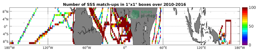
Figure 4: Number of SSS match-ups between TSG-GOSUD-Research-vessel SSS and the SMOS-L3-CATDS-CECOS-LOCEAN-V3-18DAYS-25KM SSS product for the Equatorial Ocean 10N-10S Pi-MEP region over 1^\circ \times 1^\circ boxes and for the full satellite product period.
