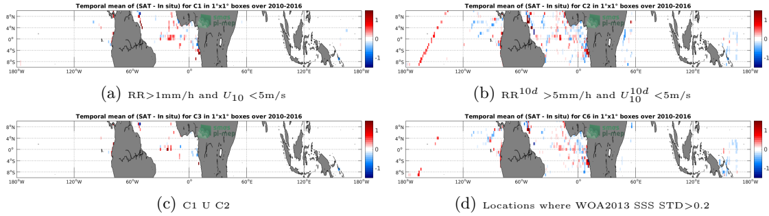
Figure 12: Temporal mean gridded over spatial boxes of size 1^\circ \times 1^\circ of \Delta SSS (SMOS-L3-CATDS-CECOS-LOCEAN-V3-18DAYS-25KM - TSG-GOSUD-Research-vessel) for 4 different subdatasets corresponding to: RR >1 mm/h and U_{10} < 5 m/s (a), RR ^{10d} > 5 mm/h and U_{10}^{10d} < 5 m/s (b), C1 U C2 (c), Locations where WOA2013 SSS STD >0.2 (d).
