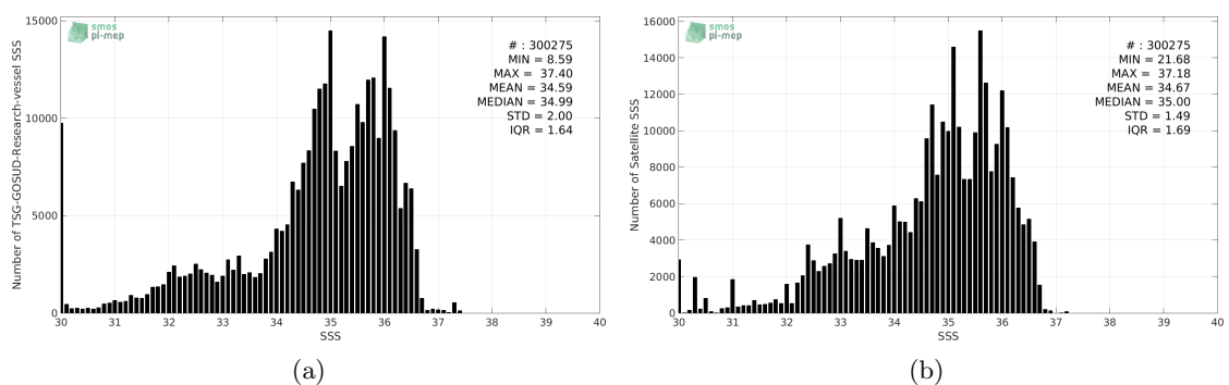
Figure 2: Histograms of SSS from TSG-GOSUD-Research-vessel (a) and SMOS-L3-CATDS-CECOS-LOCEAN-V3-18DAYS-25KM (b) considering all match-up pairs per bins of 0.1 over the Equatorial Ocean 10N-10S Pi-MEP region and for the full satellite product period.
