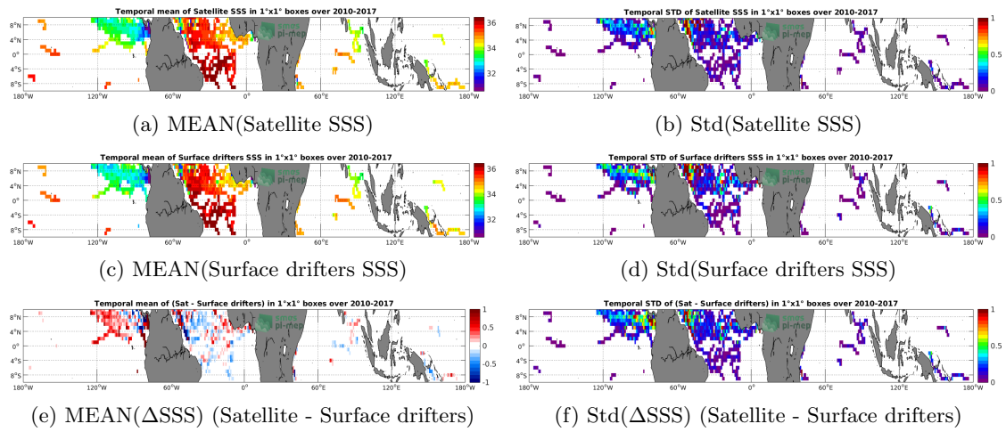
Figure 5: Temporal mean (left) and Std (right) of SSS from SMOS-L3-CATDS-CECOS-LOCEAN-V3-18DAYS-25KM (top), Surface drifters (middle), and of \Delta SSS (Satellite - Surface drifters). Only match-up pairs are used to generate these maps.
