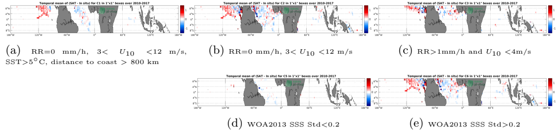
Figure 11: Temporal mean gridded over spatial boxes of size 1^\circ \times 1^\circ of \Delta SSS (SMOS-L3-CATDS-CECOS-LOCEAN-V3-18DAYS-25KM - Surface drifters) for 5 different subdatasets corresponding to: RR=0 mm/h, 3 < U_{10} < 12 m/s, SST > 5^\circ C , distance to coast > 800 km (a), RR=0 mm/h, 3 < U_{10} < 12 m/s (b), RR > 1 mm/h and U_{10} < 4 m/s (c), WOA2013 SSS Std < 0.2 (d), WOA2013 SSS Std > 0.2 (e).
