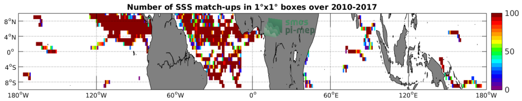
Figure 3: Number of SSS match-ups between Surface drifters SSS and the SMOS-L3-CATDS-CECOS-LOCEAN-V3-18DAYS-25KM SSS product for the Equatorial Ocean 10N-10S Pi-MEP region over 1°x1° boxes and for the full satellite product period.
