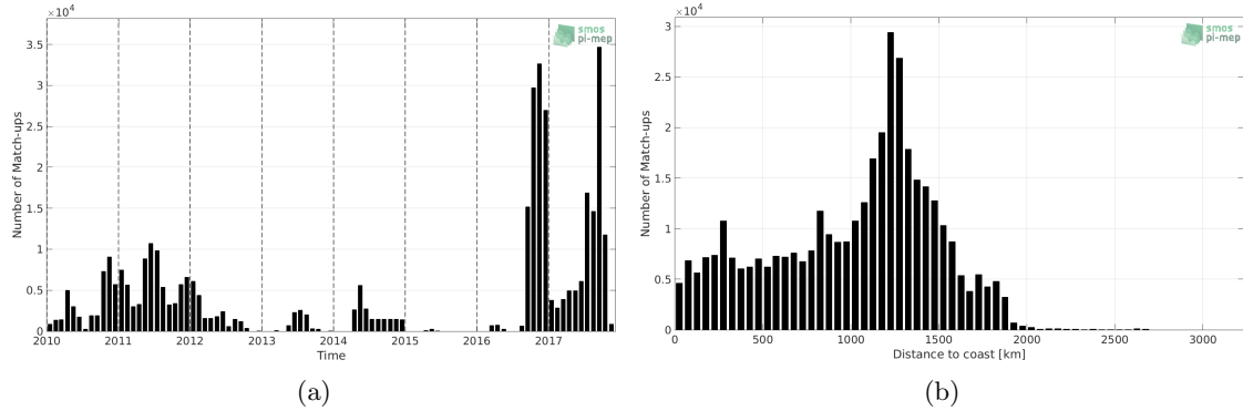
Figure 1: Number of match-ups between Surface drifters and SMOS-L3-CATDS-CECOS-LOCEAN-V3-18DAYS-25KM SSS as a function of time (a) and as function of the distance to coast (b) over the Equatorial Ocean 10N-10S Pi-MEP region and for the full satellite product period.
