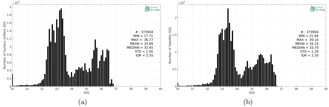
Figure 2: Histograms of SSS from Surface drifters (a) and SMOS-L3-CATDS-CECOS-LOCEAN-V3-18DAYS-25KM (b) considering all match-up pairs per bins of 0.1 over the Equatorial Ocean 10N-10S Pi-MEP region and for the full satellite product period.
