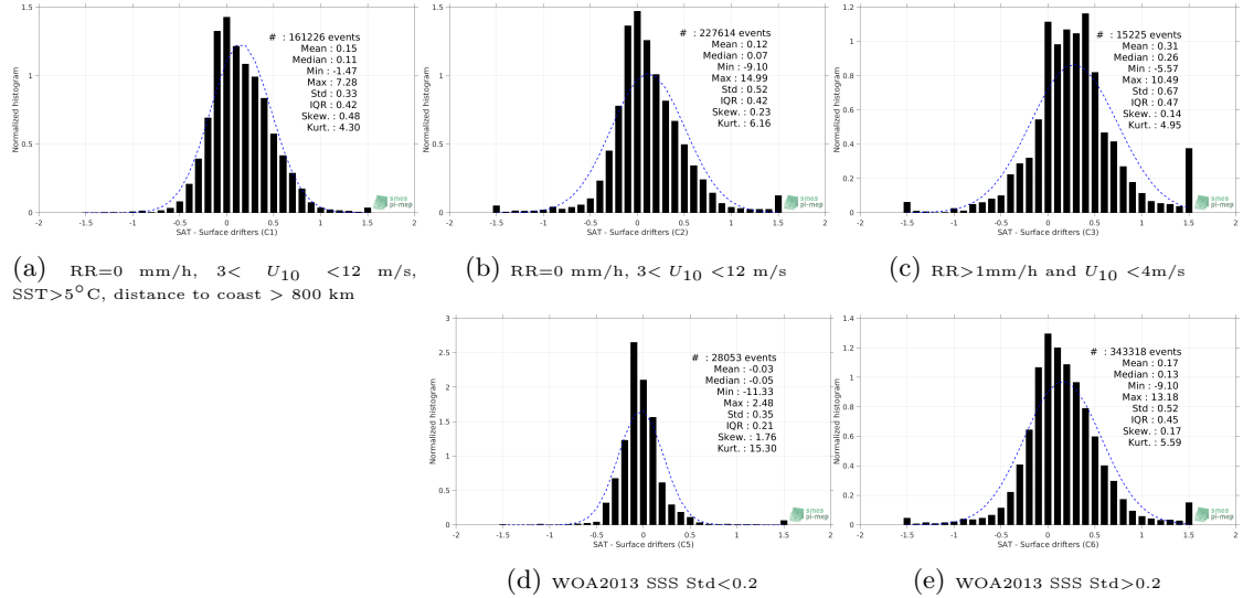
Figure 12: Normalized histogram of \Delta SSS (SMOS-L3-CATDS-CECOS-LOCEAN-V3-18DAYS-25KM - Surface drifters) for 5 different subdatasets corresponding to: RR=0 mm/h, 3 < U_{10} < 12 m/s, SST > 5^\circ C , distance to coast > 800 km (a), RR=0 mm/h, 3 < U_{10} < 12 m/s (b), RR > 1 mm/h and U_{10} < 4 m/s (c), WOA2013 SSS Std < 0.2 (d), WOA2013 SSS Std > 0.2 (e).
