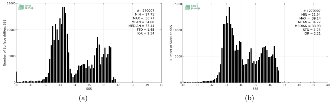
Figure 2: Histograms of SSS from Surface drifters (a) and SMOS-L3-CATDS-CECOS-LOCEAN-V3-18DAYS-25KM (b) considering all match-up pairs per bins of 0.1 over the Equatorial Ocean 10N-10S Pi-MEP region and for the full satellite product period.
