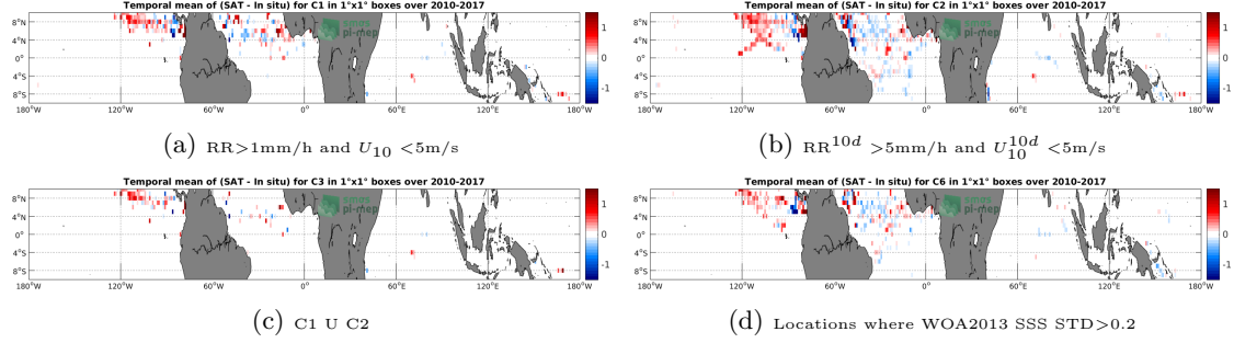
Figure 11: Temporal mean gridded over spatial boxes of size 1^\circ \times 1^\circ of \Delta SSS (SMOS-L3-CATDS-CECOS-LOCEAN-V3-18DAYS-25KM - Surface drifters) for 4 different subdatasets corresponding to: RR > 1\text{mm/h} and U_{10} < 5\text{m/s} (a), RR^{10d} > 5\text{mm/h} and U_{10}^{10d} < 5\text{m/s} (b), C1 U C2 (c), Locations where WOA2013 SSS STD > 0.2 (d).
