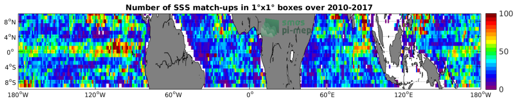
Figure 4: Number of SSS match-ups between Argo SSS and the SMOS-L3-CATDS-CECOS-LOCEAN-V3-18DAYS-25KM SSS product for the Equatorial Ocean 10N-10S Pi-MEP region over 1°x1° boxes and for the full satellite product period.
