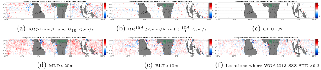
Figure 12: Temporal mean gridded over spatial boxes of size 1^\circ \times 1^\circ of \Delta\text{SSS} (SMOS-L3-CATDS-CECOS-LOCEAN-V3-18DAYS-25KM - Argo) for 6 different subdatasets corresponding to: \text{RR} > 1\text{mm/h} and U_{10} < 5\text{m/s} (a), \text{RR}^{10d} > 5\text{mm/h} and U_{10}^{10d} < 5\text{m/s} (b), C1 U C2 (c), \text{MLD} < 20\text{m} (d), \text{BLT} > 10\text{m} (e), Locations where WOA2013 SSS \text{STD} > 0.2 (f).
