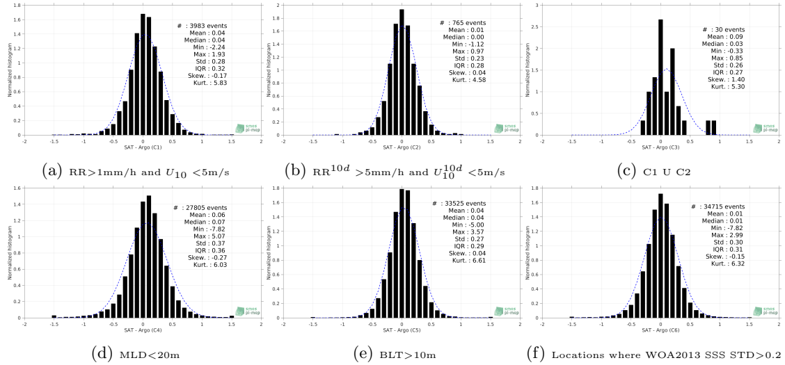
Figure 13: Normalized histogram of \Delta\text{SSS} (SMOS-L3-CATDS-CECOS-LOCEAN-V3-18DAYS-25KM - Argo) for 6 different subdatasets corresponding to: \text{RR} > 1\text{mm/h} and U_{10} < 5\text{m/s} (a), \text{RR}^{10d} > 5\text{mm/h} and U_{10}^{10d} < 5\text{m/s} (b), C1 U C2 (c), \text{MLD} < 20\text{m} (d), \text{BLT} > 10\text{m} (e), Locations where WOA2013 SSS \text{STD} > 0.2 (f).
