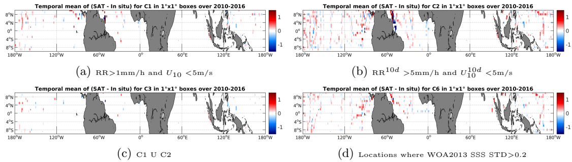
Figure 12: Temporal mean gridded over spatial boxes of size 1^\circ \times 1^\circ of \Delta SSS (SMOS-L3-CATDS-CECOS-LOCEAN-V2.1-9DAYS-25KM - TSG-SAMOS) for 4 different subdatasets corresponding to: RR > 1\text{mm/h} and U_{10} < 5\text{m/s} (a), RR^{10d} > 5\text{mm/h} and U_{10}^{10d} < 5\text{m/s} (b), C1 U C2 (c), Locations where WOA2013 SSS STD > 0.2 (d).
