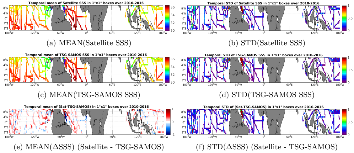
Figure 6: Temporal mean (left) and STD (right) of SSS from SMOS-L3-CATDS-CECOS-LOCEAN-V2.1-9DAYS-25KM (top), TSG-SAMOS (middle), and of \Delta SSS (Satellite - TSG-SAMOS). Only match-up pairs are used to generate these maps.
