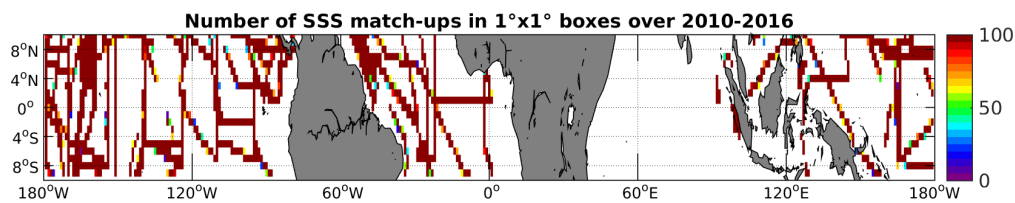
Figure 4: Number of SSS match-ups between TSG-SAMOS SSS and the SMOS-L3-CATDS-CECOS-LOCEAN-V2.1-9DAYS-25KM SSS product for the Equatorial Ocean 10N-10S Pi-MEP region over 1^\circ \times 1^\circ boxes and for the full satellite product period.
