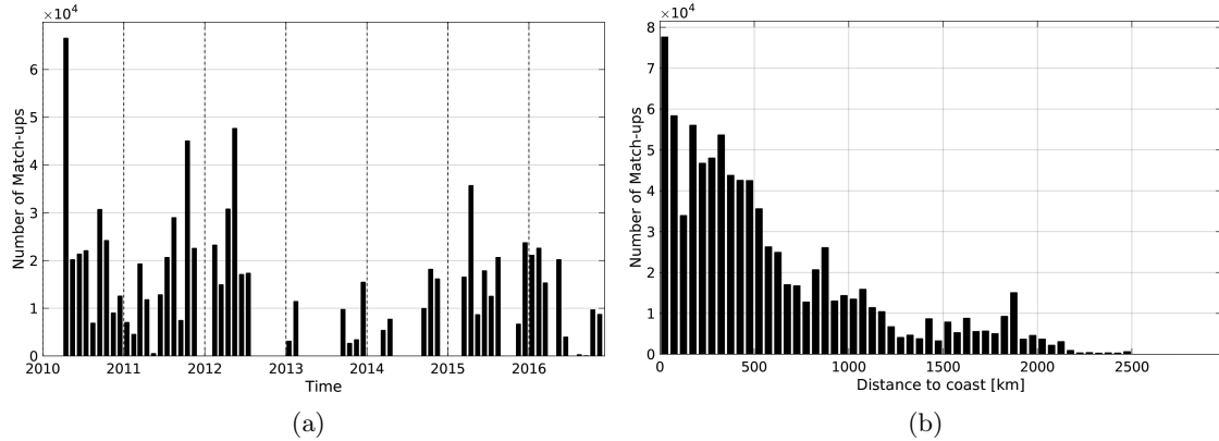
Figure 1: Number of match-ups between TSG-SAMOS and SMOS-L3-CATDS-CECOS-LOCEAN-V2.1-9DAYS-25KM SSS as a function of time (a) and as function of the distance to coast (b) over the Equatorial Ocean 10N-10S Pi-MEP region and for the full satellite product period.
