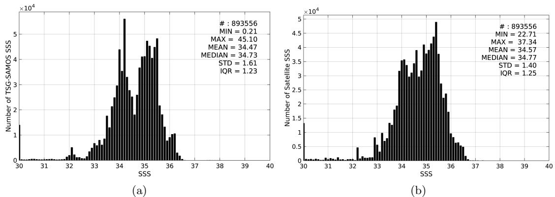
Figure 2: Histograms of SSS from TSG-SAMOS (a) and SMOS-L3-CATDS-CECOS-LOCEAN-V2.1-9DAYS-25KM (b) considering all match-up pairs per bins of 0.1 over the Equatorial Ocean 10N-10S Pi-MEP region and for the full satellite product period.
