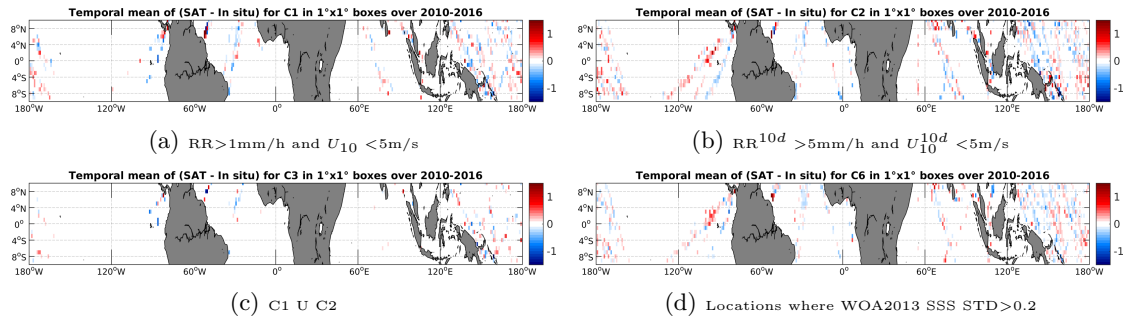
Figure 12: Temporal mean gridded over spatial boxes of size 1^\circ \times 1^\circ of \Delta SSS (SMOS-L3-CATDS-CECOS-LOCEAN-V2.1-9DAYS-25KM - TSG-LEGOS-DM) for 4 different subdatasets corresponding to: RR > 1\text{mm/h} and U_{10} < 5\text{m/s} (a), RR^{10d} > 5\text{mm/h} and U_{10}^{10d} < 5\text{m/s} (b), C1 U C2 (c), Locations where WOA2013 SSS STD > 0.2 (d).
