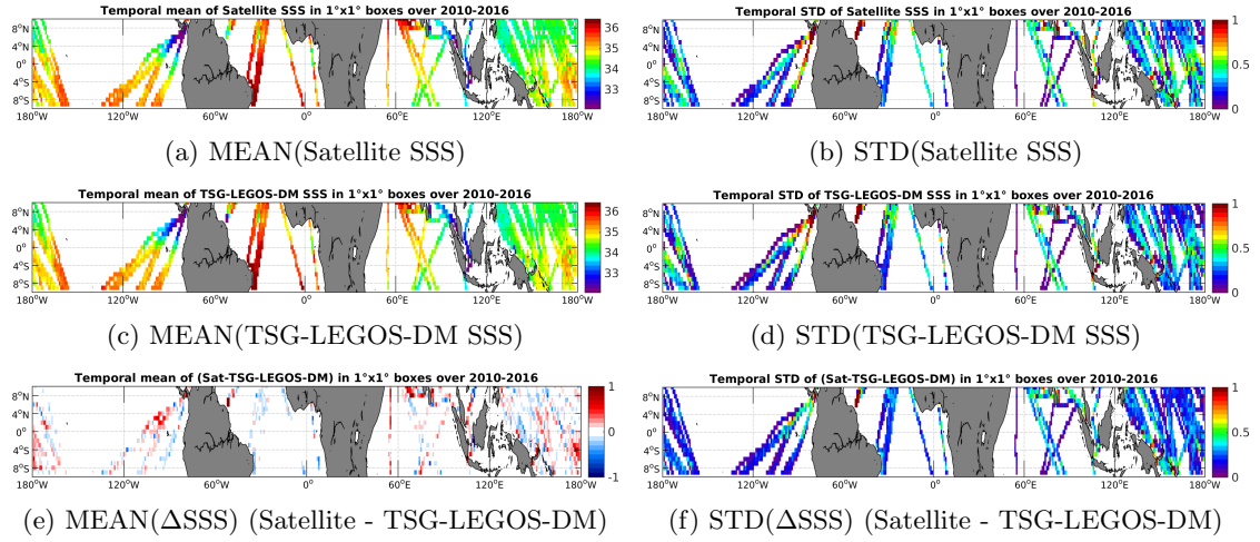
Figure 6: Temporal mean (left) and STD (right) of SSS from SMOS-L3-CATDS-CECOS-LOCEAN-V2.1-9DAYS-25KM (top), TSG-LEGOS-DM (middle), and of \Delta SSS (Satellite - TSG-LEGOS-DM). Only match-up pairs are used to generate these maps.
