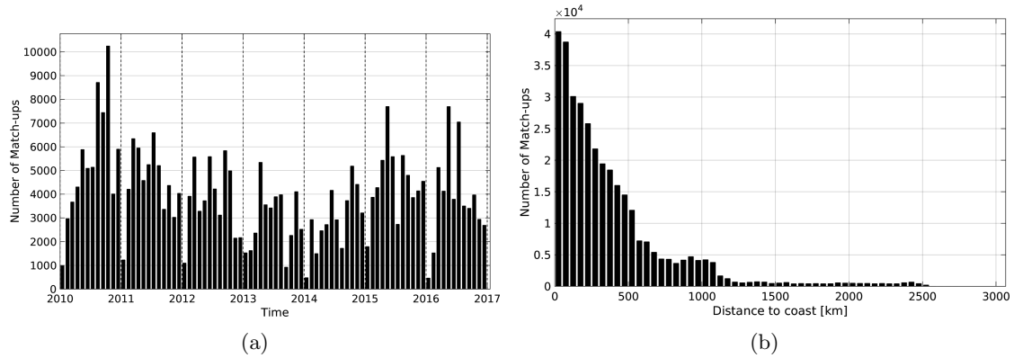
Figure 1: Number of match-ups between TSG-LEGOS-DM and SMOS-L3-CATDS-CECOS-LOCEAN-V2.1-9DAYS-25KM SSS as a function of time (a) and as function of the distance to coast (b) over the Equatorial Ocean 10N-10S Pi-MEP region and for the full satellite product period.
