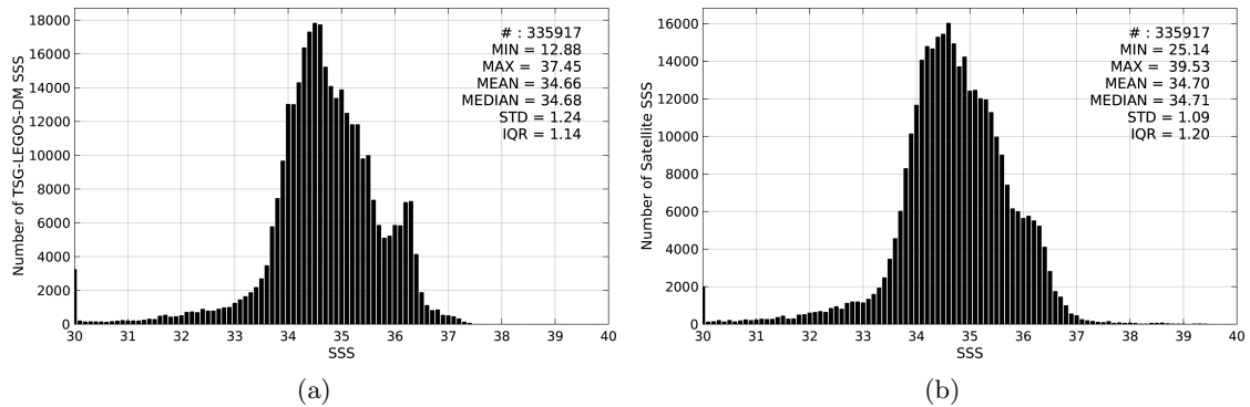
Figure 2: Histograms of SSS from TSG-LEGOS-DM (a) and SMOS-L3-CATDS-CECOS-LOCEAN-V2.1-9DAYS-25KM (b) considering all match-up pairs per bins of 0.1 over the Equatorial Ocean 10N-10S Pi-MEP region and for the full satellite product period.
