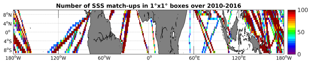
Figure 4: Number of SSS match-ups between TSG-LEGOS-DM SSS and the SMOS-L3-CATDS-CECOS-LOCEAN-V2.1-9DAYS-25KM SSS product for the Equatorial Ocean 10N-10S Pi-MEP region over 1^\circ \times 1^\circ boxes and for the full satellite product period.
