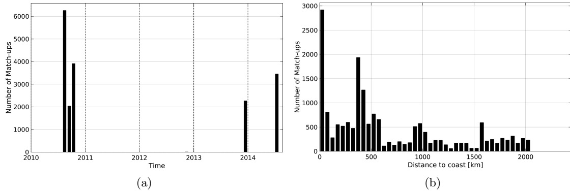
Figure 1: Number of match-ups between TSG-GOSUD-Sailing-ship and SMOS-L3-CATDS-CECOS-LOCEAN-V2.1-9DAYS-25KM SSS as a function of time (a) and as function of the distance to coast (b) over the Equatorial Ocean 10N-10S Pi-MEP region and for the full satellite product period.
