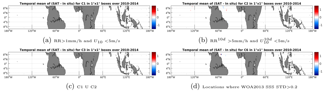
Figure 12: Temporal mean gridded over spatial boxes of size 1^\circ \times 1^\circ of \Delta SSS (SMOS-L3-CATDS-CECOS-LOCEAN-V2.1-9DAYS-25KM - TSG-GOSUD-Sailing-ship) for 4 different subdatasets corresponding to: RR > 1\text{mm/h} and U_{10} < 5\text{m/s} (a), RR^{10d} > 5\text{mm/h} and U_{10}^{10d} < 5\text{m/s} (b), C1 U C2 (c), Locations where WOA2013 SSS STD > 0.2 (d).
