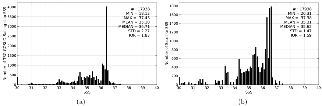
Figure 2: Histograms of SSS from TSG-GOSUD-Sailing-ship (a) and SMOS-L3-CATDS-CECOS-LOCEAN-V2.1-9DAYS-25KM (b) considering all match-up pairs per bins of 0.1 over the Equatorial Ocean 10N-10S Pi-MEP region and for the full satellite product period.
