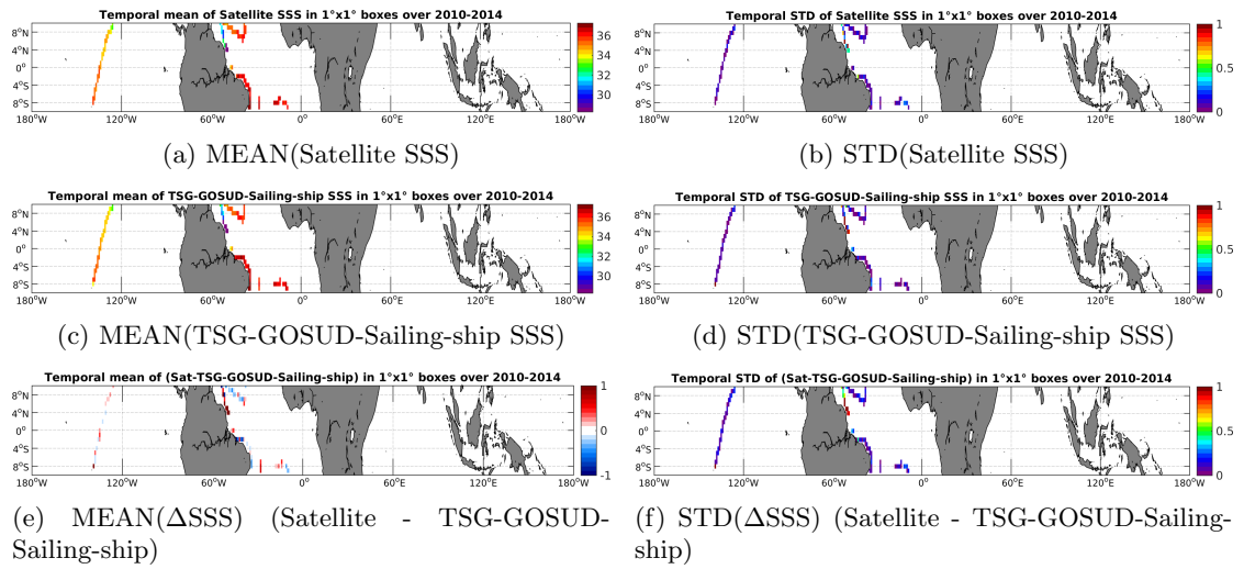
Figure 6: Temporal mean (left) and STD (right) of SSS from SMOS-L3-CATDS-CECOS-LOCEAN-V2.1-9DAYS-25KM (top), TSG-GOSUD-Sailing-ship (middle), and of \Delta SSS (Satellite - TSG-GOSUD-Sailing-ship). Only match-up pairs are used to generate these maps.
